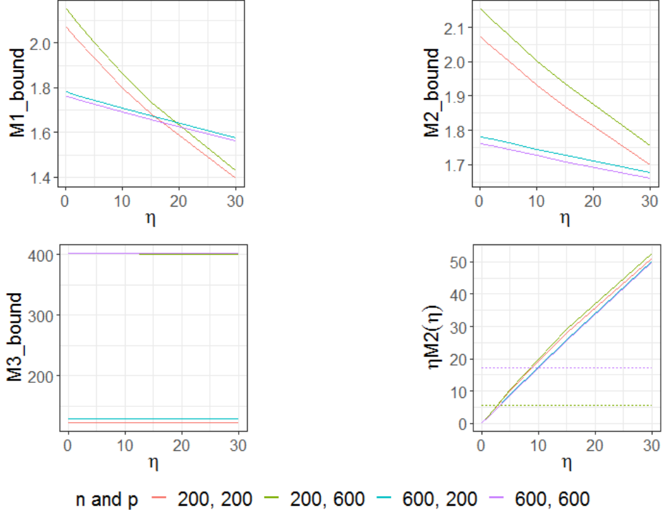
Figure 3: Top left: Average of \lambda_{\max}(H_A H_A') in (19) as a function of \eta . Top right: Average of \lambda_{\max}\left(\left(\mathcal{C}_{11}^{n,\Sigma}\right)^{-1}\right) in (20) as a function of \eta . Bottom left: Average of \lambda_{\max}(H_B H_B') in (21) as a function of \eta . Bottom right: Average of the left (resp. right) part of (24) in plain (resp. dashed) line. The averages are obtained from 10 replications. Here q = 10 .
