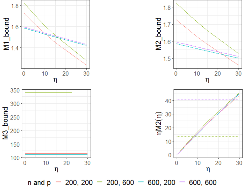
Figure 2: Top left: Average of \lambda_{\max}(H_A H_A') in (19) as a function of \eta . Top right: Average of \lambda_{\max}\left(\left(\mathcal{C}_{11}^{n,\Sigma}\right)^{-1}\right) in (20) as a function of \eta . Bottom left: Average of \lambda_{\max}(H_B H_B') in (21) as a function of \eta . Bottom right: Average of the left (resp. right) part of (24) in plain (resp. dashed) line. The averages are obtained from 10 replications. Here q = 5 .
