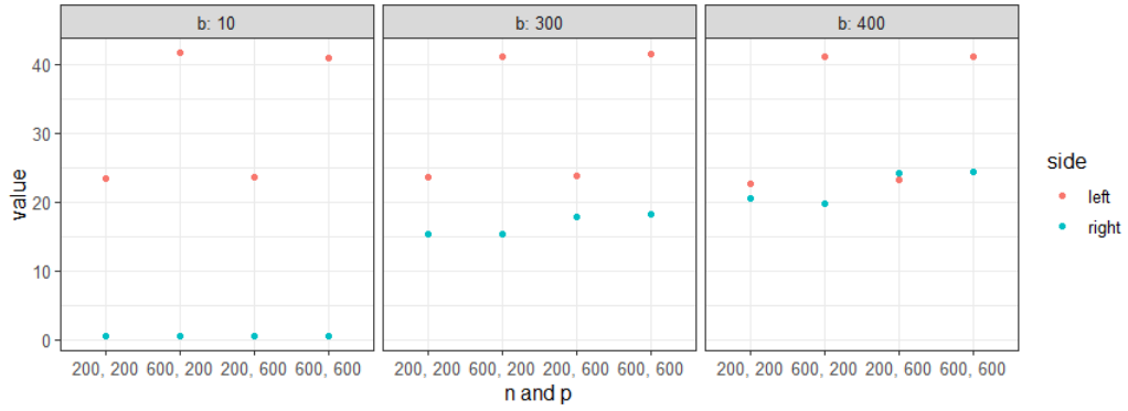
Figure 5: Average of the left-hand (resp. right-hand) side of the second part of (15) in red (resp. blue) for q = 10 .
