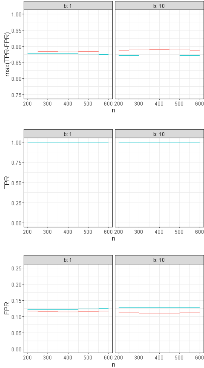
Figure 7: Average of \max(\text{TPR}-\text{FPR}) and the corresponding TPR and FPR for gEN (in red) and Elastic Net (in blue) with p = 400 .
