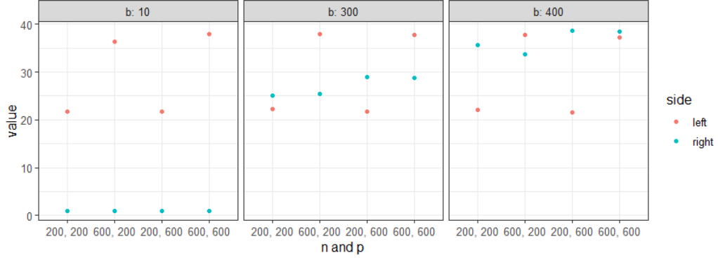
Figure 4: Average of the left-hand (resp. right-hand) side of the second part of (15) in red (resp. blue) for q = 5 .
