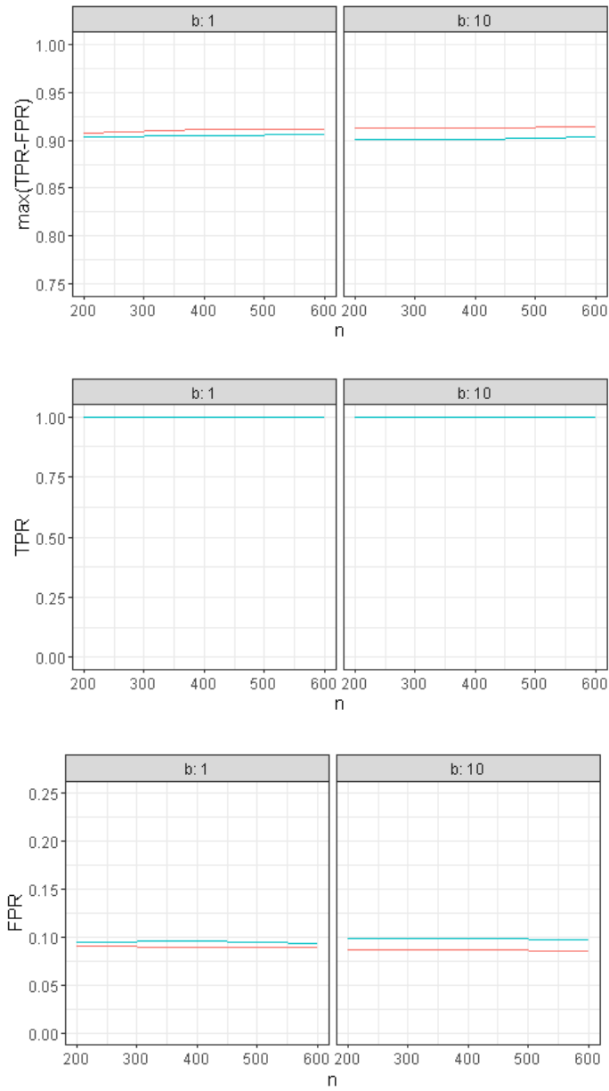
Figure 8: Average of \max(\text{TPR}-\text{FPR}) and the corresponding TPR and FPR for gEN (in red) and Elastic Net (in blue) with p = 600 .
