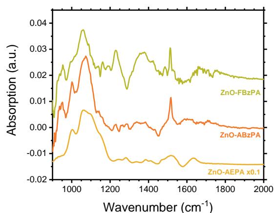
Figure 3: ATR-FTIR spectra of ZnO-AEPA, ZnO-ABzPA and ZnO-FBzPA. The Si-ZnO substrates were taken as reference. Note that absorption of ZnO-AEPA is multiplied by 0.1.
