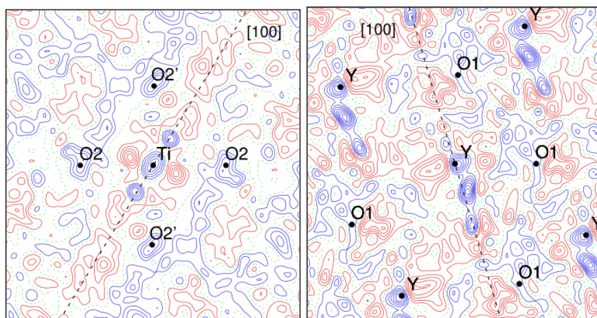
Figure 4 Residual charge density around titanium and yttrium atoms. Contours are 0.10 e/\text{Å}^3 . Green dotted contours are zero level, red ones are negative, blue ones are positive. The [100] direction is shown by black dotted lines. \sin(\theta)/\lambda < 1.2 \text{Å}^{-1} .
