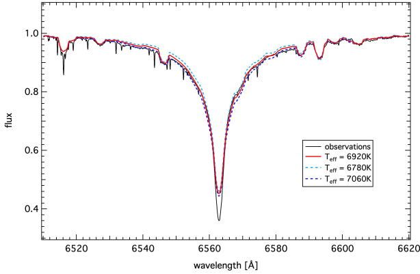
Fig. 6. Region of the H \alpha line for \beta Cas: the observed spectrum is shown in black and the calculated synthetic spectrum with the final adopted parameters of T_{\text{eff}} = 6920 K and \log g = 3.53 cgs in red. The dashed light blue line represents a synthetic spectrum with a 140 K lower T_{\text{eff}} and the dashed dark blue line a synthetic spectrum with a 140 K higher T_{\text{eff}} .
