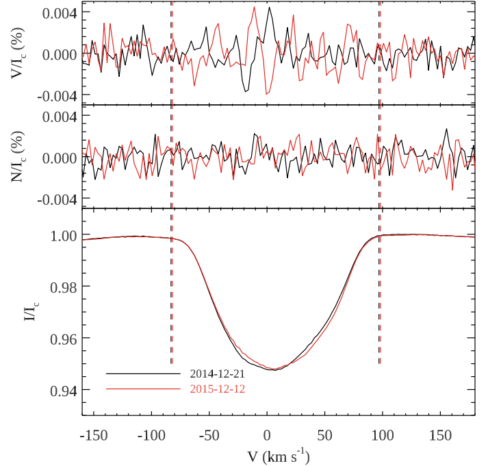
Fig. 8. Representative LSD Stokes I , V , and null profiles of \beta Cas. The two sets of profiles shown here correspond to the Narval observations obtained on 21 December 2014 (data set #4 in Table 2) and 12 December 2015 (data set #18). The vertical dashed lines indicate measurement windows adopted in Sect. 5.2 for these two observations.
