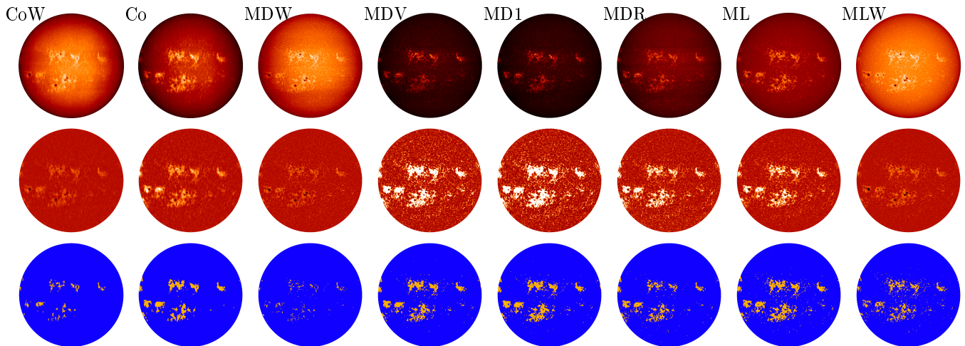
Fig. 12. Examples of observations taken on the same date (04 July 2014) from the various datasets analysed in this study with images not centred at the core of the Ca II K line along with those from the same observatories centred at the core of the Ca II K line. Shown are images from the CoW, Co, MDW, MDV, MD1, MDR, ML, MLW datasets after the preprocessing to identify the disc and re-sample them to account for the disc ellipticity ( top row ), after CLV-compensation ( middle row ), and after the identification of plage ( bottom row ). The images have been aligned to show the solar north pole at the top. The raw images are shown to their entire range of values, the CLV-compensated images are shown in the range [-0.5, 0.5] , while in the masks, the plage regions are shown in orange and the quiet Sun and network regions in blue. We stress that the same threshold was used for all datasets to identify the plage regions, which is why the different datasets seem to provide rather different ranges of plage coverage.
