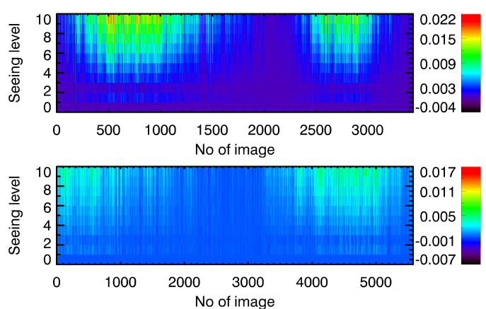
Fig. 11. Colour-coded difference in fractional plage areas derived from RP1 ( top ) and MD1 ( bottom ) images downgraded to simulate effects of seeing and those derived from the original RP1 and MD1 images, respectively. The MD1 data used here are only those taken with a CCD camera between 2002 and 2017. Each row (column) of boxes shows results derived from a given observation (width of the smoothing Gaussian function). See Sect. 4 for details.
