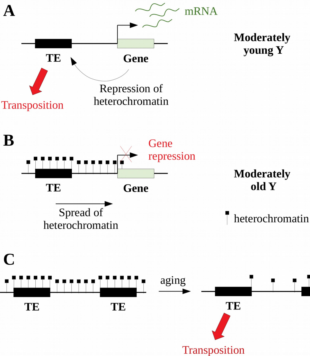
Figure 2: Epigenetics of Y degeneration and Y toxicity. A) In moderately young Y chromosomes, numerous actively transcribed genes prevent the formation of heterochromatin on nearby TEs. This may lead to active TE transposition. B) In moderately old Y chromosomes, few Y genes are surrounded by TEs. Heterochromatin marks spread to genes and prevent their expression, leading to further Y degeneration. C) Heterochromatin marks get lost through aging leading to active transposition of TEs. This phenomenon will be particularly prevalent in males with a Y chromosome and lead to Y toxicity.
