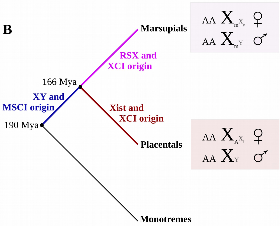
Figure 3: Evolution of the epigenetics of dosage compensation in Drosophila and mammals.
