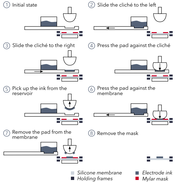
Figure 7: Pad-printing procedure used to apply the soft conductive electrodes. The steps 1-8 are then repeated on the other side of the membrane to apply the second electrode.
