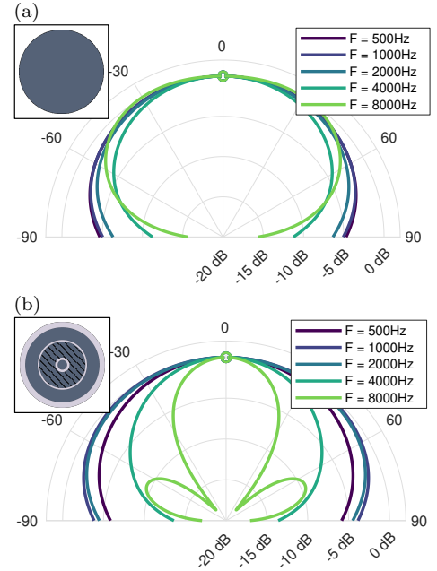
Figure 12: Near field directivity of the inflated DE loudspeaker, computed by the finite element model on a circle of 5 cm diameter centered on the membrane, and normalized by the level on axis. (a) Initial design, with electrode 1 (see table 1). (b) Optimal electrode obtained when the second electrode ring is actuated out of phase, shown in fig. 11(b).
