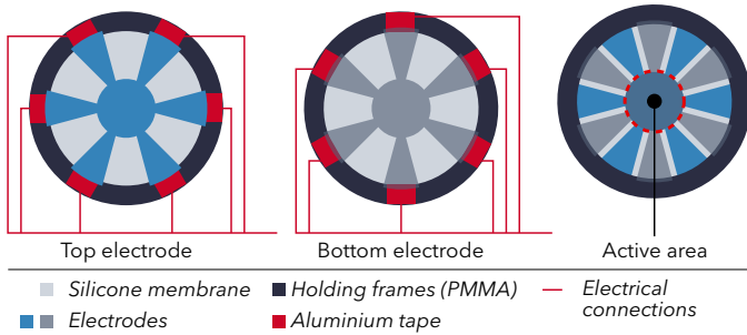
Figure 6: Design of the electrodes and of the electrical connections. The active area is enclosed by the red dashed circle.
