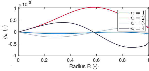
Figure 10: Modal participation factor as a function of the membrane radius for the first four modes.
