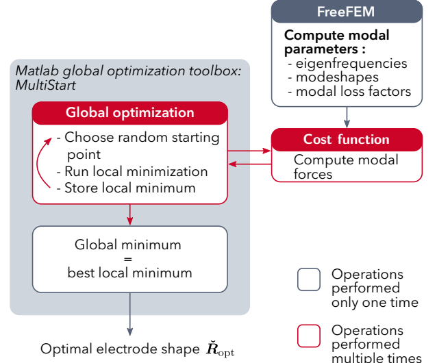
Figure 5: Flowchart of the optimization procedure.
