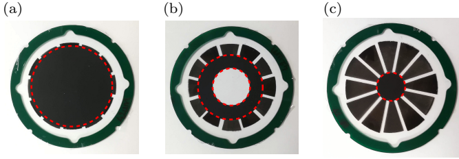
Figure 8: Manufactured membranes with the three electrode shapes defined in table 1. The active areas are enclosed by the red dashed circles. (a) Electrode 1: initial design. (b) Electrode 2: maximize radiation of mode 2. (c) Electrode 3: minimize radiation of mode 2.
