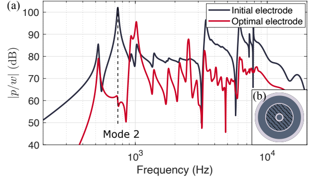
Figure 11: (a) Computed radiation of the DE loudspeaker with electrode 4, for cost function J . (b) Optimal electrode shape. The second electrode ring (hatched) is driven out of phase of the two other rings.
