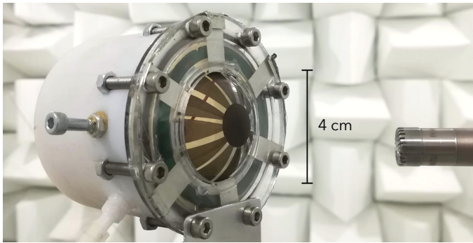
Figure 2: Picture of an inflated DE loudspeaker prototype during acoustical measurements in the anechoic chamber of ENSTA.
