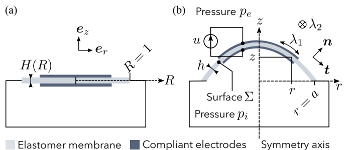
Figure 3: Model of an inflated DE membrane, and definition of the needed variables. (a) Reference configuration: the membrane is flat and at rest. Variables in the reference configuration are written with capital letters. (b) Deformed configuration: the membrane is inflated with the pressure p_i and a high voltage u is applied.
