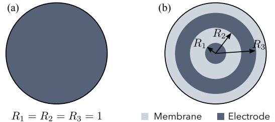
Figure 4: Definition of the optimized parameters: the non-dimensional radii R_i of the different electrode rings. Here, an electrode with 3 radii is shown. (a) Initial electrode (where the second electrode between R_2 and R_3 is infinitely narrow). (b) Optimized electrode.
