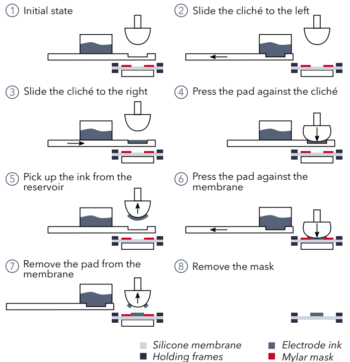
Figure 7: Pad-printing procedure used to apply the soft conductive electrodes. The steps 1-8 are then repeated on the other side of the membrane to apply the second electrode.
