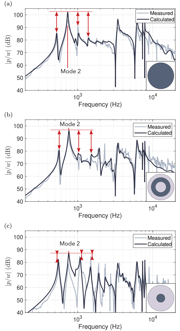
Figure 9: Transfer function between the radiated acoustic pressure at 1 m on axis and the excitation signal. The electrode shape is shown in the bottom right corner. (a) Electrode 1. (b) Electrode 2. (c) Electrode 3.
