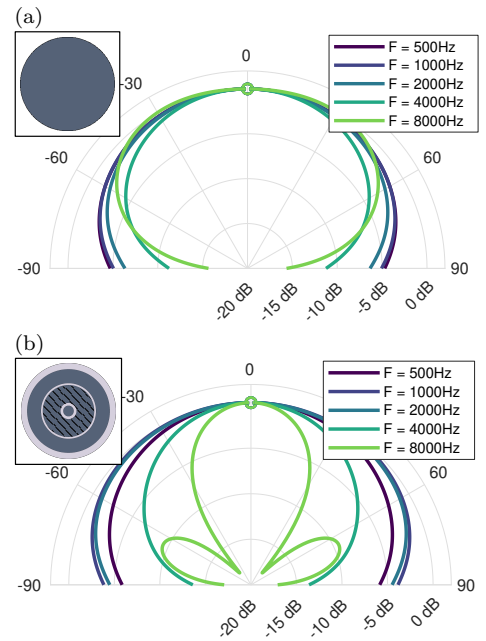
Figure 12: Near field directivity of the inflated DE loudspeaker, computed by the finite element model on a circle of 5 cm diameter centered on the membrane, and normalized by the level on axis. (a) Initial design, with electrode 1 (see table 1). (b) Optimal electrode obtained when the second electrode ring is actuated out of phase, shown in fig. 11(b).
