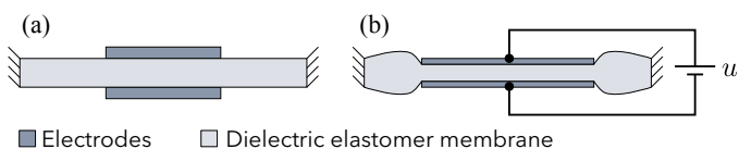
Figure 1: Principle of dielectric elastomer actuators. (a) Initial state. (b) Deformed state, when a high voltage u is applied.
