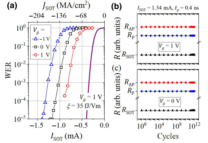
FIG. 9. (a) WER of 10^5 events for the AP-P transition at t_p = 0.4 ns. Purple curve predicts the WER for \xi = 35 fJ/Vm at V_g = 1 V, which is required to achieve full selectivity. (b) Endurance tests of 10^{12} cycles at applied SOT current I_{\text{SOT}} = 1.34 mA and t_p = 0.4 ns with 50 MHz repetition rate for (b) selected cell V_g = 1 V and (c) unselected cell V_g = 0 V.
