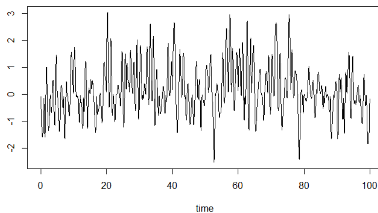
Figure 3. One trajectory.
