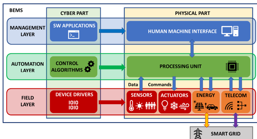
Figure 4. BEMS conceptual architecture.
