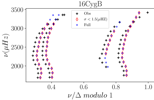
Fig. C.2. Échelle diagram of 16 Cygni B comparing optimal reference model with full set of frequencies (blue circles) from (Davies et al. 2015; black crosses) with the optimal model with a set restricted to frequencies with uncertainties lower than 1.5 \mu\text{Hz} (red diamonds).
