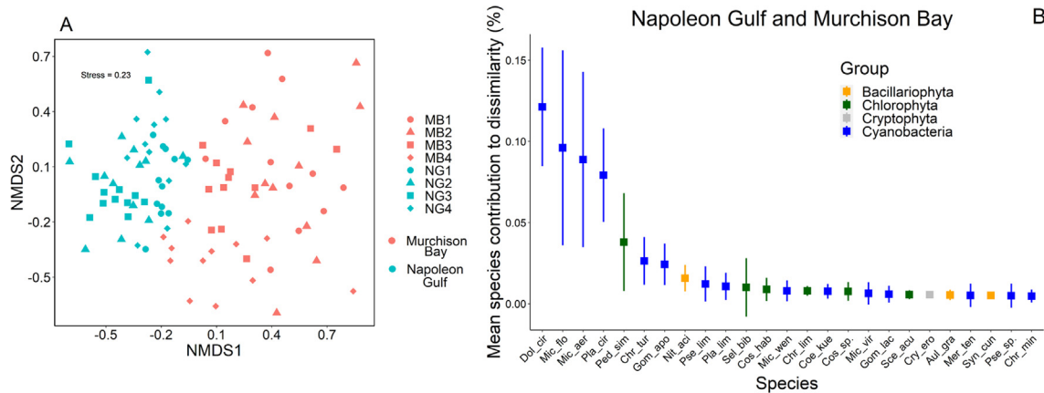
Fig. 5. Differences in structure of the phytoplankton communities and contributing taxa. Plot A: nMDS ordination of the communities performed on Bray-Curtis dissimilarities matrix using relative biovolume matrices (stress = 0.23). Plot B: Average taxa contribution to dissimilarity between phytoplankton communities from the two bays. The values are averaged across all pairs of communities. Note: Full names of the phytoplankton taxa are in ESM Table S3.
