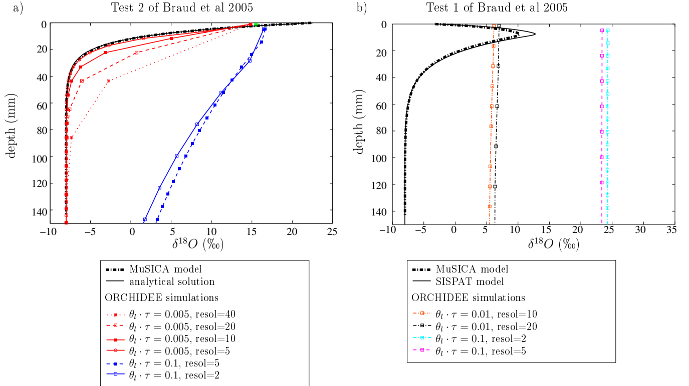
Figure E.15: Vertical profile of soil water \delta^{18}O in idealized cases described by [Braud et al., 2005]. a) The soil column evaporates at its top and is permanently refilled at the bottom by a water with \delta^{18}O = -8\text{‰} . b) The soil column is evaporated progressively until its soil water content is only 20%. See appendix C.2 for more details. Simulations using the soil profile module of the isotopic version of ORCHIDEE (colors) with different parameters and vertical resolution are compared with the more sophisticated MuSICA and SiSPAT models and with an analytical solution. For \theta_i \cdot \tau = 0.005 , the vertical resolution for ORCHIDEE is 0.15 mm for the first layer and 0.75 mm (resol=5), 1.5 mm (resol=10), 3 mm (resol=20) or 6 mm (resol=40) for the other layers. For \theta_i \cdot \tau = 0.01 , the vertical resolution for ORCHIDEE is 0.21 mm for the first layer and 2.12 mm (resol=10) or 4.24 mm (resol=20) for the other layers. For \theta_i \cdot \tau = 0.1 , the vertical resolution for ORCHIDEE is 0.67 mm for the first layer and from 1.34 mm (resol=2) to 3.35 mm (resol=5) for the other layers.
