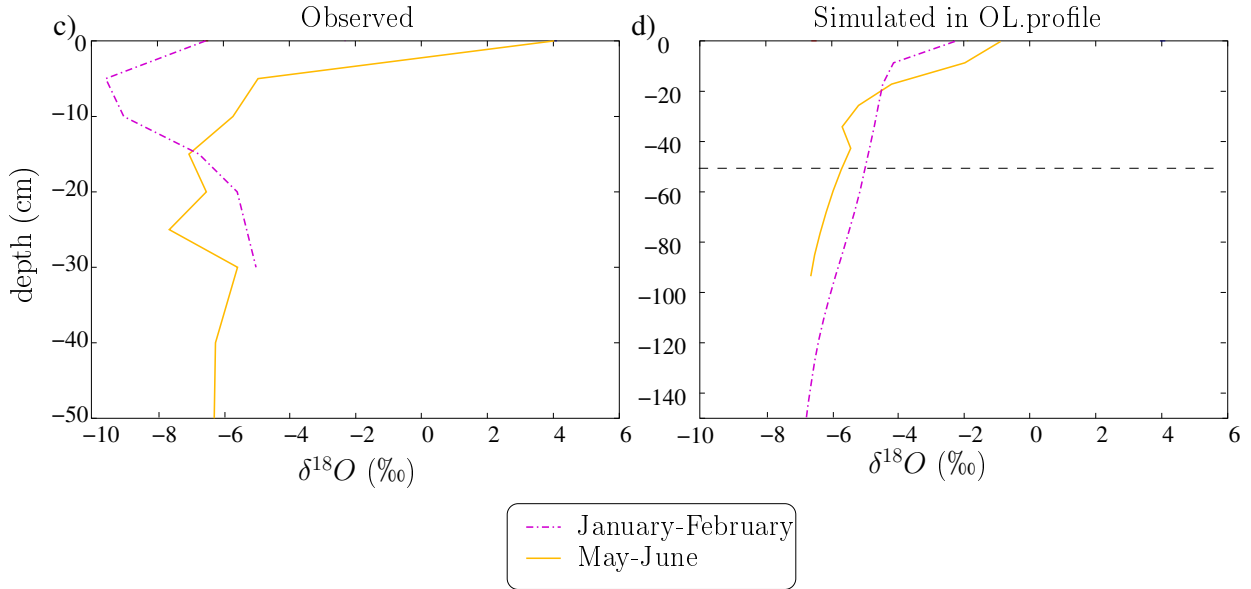
Figure E.6: Vertical profiles of soil \delta^{18}O measured (a,c) and simulated by ORCHIDEE for the control offline simulations (b,d) on the Bray site (a,b) and the Yatir sites (b,d). Beware that the y-scales for observations and simulations are different. This is because the representation of the soil water content is very rudimentary in the ORCHIDEE model, preventing any quantitative comparison of measured and simulated soil depth. The horizontal black dashed line represents the bottom of the observed profiles. Model outputs are sampled at the same time as the data. For the Yatir sites, frequent soil sampling for the same year allowed us plot representative bi-monthly averages for both measured and simulated profiles. This could not be the case for Le Bray. Some soil profiles were observed at Le Bray in 2007, but we do not show them because they are limited to the top 24 cm of the soil only.
