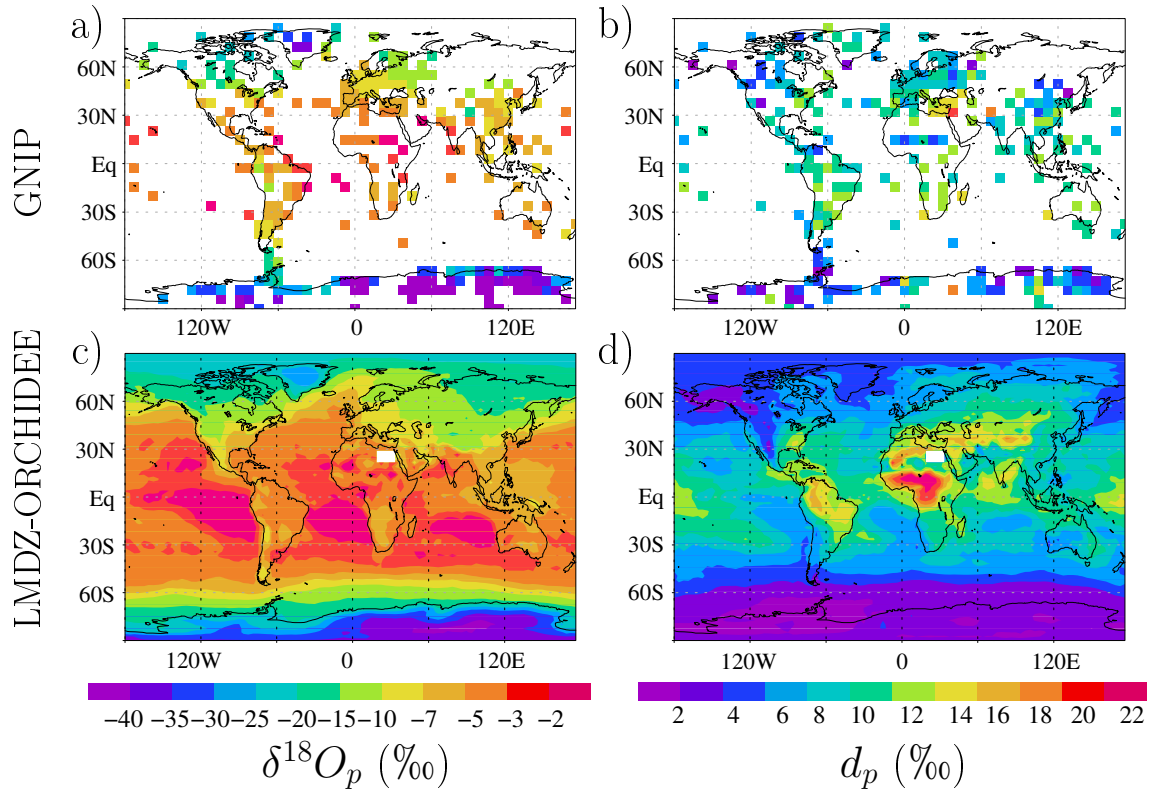
Figure E.10: a) Annual mean \delta^{18}O_p from GNIP ([Rozanski et al., 1993]), Antarctica ([Masson-Delmotte et al., 2008]) and Greenland ([Masson-Delmotte et al., 2005]) data. The data is gridded over a coarse 7.5 \times 6.5^\circ grid for visualization purposes. b) Same as a) but for annual mean d_p . c) Annual mean \delta^{18}O_p simulated by coupled LMDZ-ORCHIDEE model for the control simulation. d) same as c) but for annual mean d_p .
