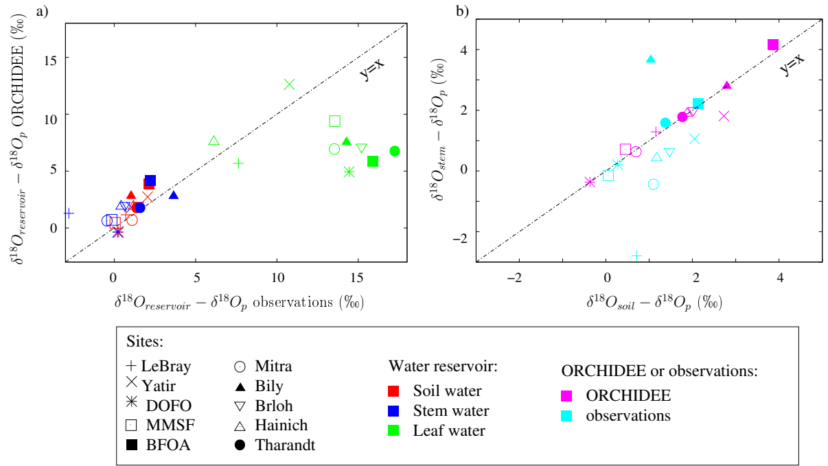
Figure E.5: a) Relationship between simulated and observed annual-mean \delta^{18}O in the soil water (red), stem water (blue) and leaf water (green), to which the precipitation-weighted annual-mean precipitation \delta^{18}O is subtracted. In the case of perfect model-data agreement, markers should fall on the y=x line. b) Relationship between the annual-mean \delta^{18}O in the soil water and in stem water, to which the precipitation-weighted annual-mean precipitation \delta^{18}O is subtracted, for both ORCHIDEE (magenta) and observations (cyan). When soil and stem water share the same \delta^{18}O , they fall on the y=x line.
