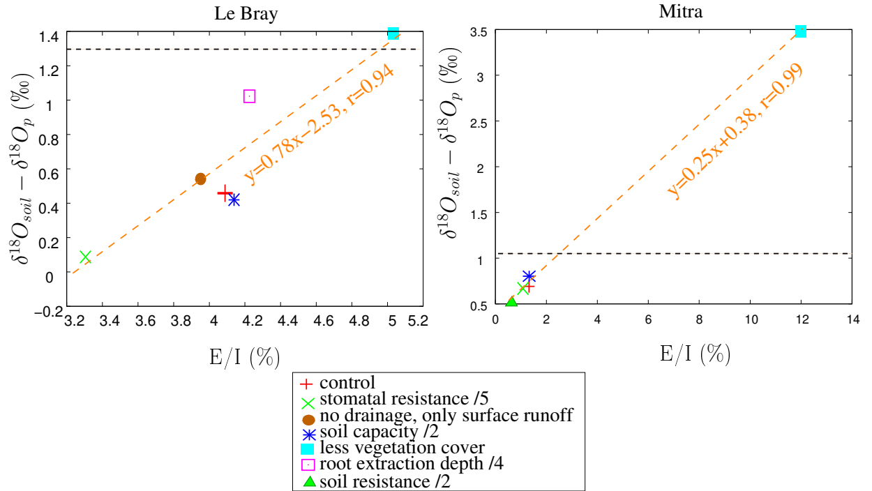
Figure E.7: Isotopic difference between soil water and precipitation ( \delta^{18}O_s - \delta^{18}O_p ), as a function of E/I (fraction of the infiltrated water that evaporates at the bare soil surface), for different sensitivity tests in ORCHIDEE. a) at Le Bray and b) at Mitra. All values are annual means. The horizontal dashed line represents the observed values for \delta^{18}O_s - \delta^{18}O_p . The orange dashed line shows the best linear fit between the different sensitivity tests.
