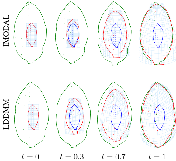
Figure 8: Basipetal growth: registration of curves and dots using IMODAL or unstructured large deformations. The source is blue, target is green and deformed source is red.
