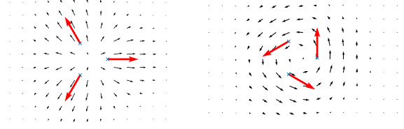
Figure 3: Local scaling (left) and local rotation (right) vector fields approximated by constrained translations generated by 3 control points each.
