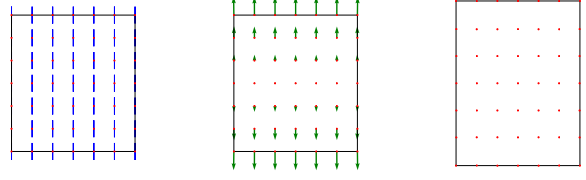
Figure 5: Vertical uniform elongation. Left: the blue (degenerate) ellipses represent the growth factor R_i D_i R_i^T with D_i = \text{diag}(0, 1) and R_i = \text{Id} for each x_i (red points). Middle: generated vector field in green. Right: infinitesimal deformation of the rectangle induced by this field.
