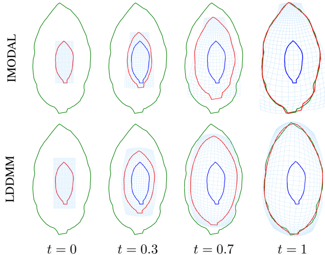
Figure 2: Basipetal growth: curves registration using IMODAL and LDDMM (unstructured large deformation). The source is blue, target is green and the deformed source is red.
