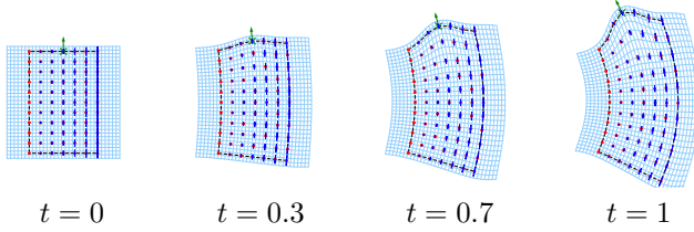
Figure 7: Example of large deformation generated by the combination of an implicit module M^1 of order 1 and a module M^2 generating a local translation. The red points are the point-component of the geometrical descriptor of M^1 , the blue (flat) ellipses represent the growth factor. The green point is the geometrical descriptor of M^2 and the green vector is its control.
