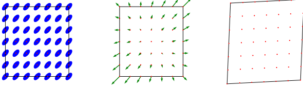
Figure 6: Uniform shearing. Left: the blue ellipses represent the growth factor R_i D_i R_i^T with D_i = \text{diag}(2, 1) and R_i = \begin{pmatrix} \cos \pi/4 & -\sin \pi/4 \\ \sin \pi/4 & \cos \pi/4 \end{pmatrix} . Middle: generated vector field in green. Right: infinitesimal deformation of the rectangle induced by this field.
