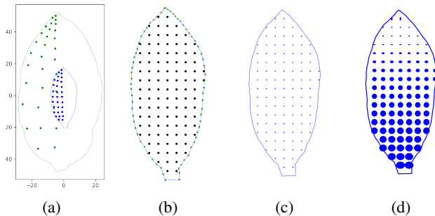
Figure 9: (a) Data extracted from Figure 1a ; (b) Initial geometrical descriptors: black (order 1) and green (order 0) ; Initialization (c) and estimation (d) of the growth factor.
