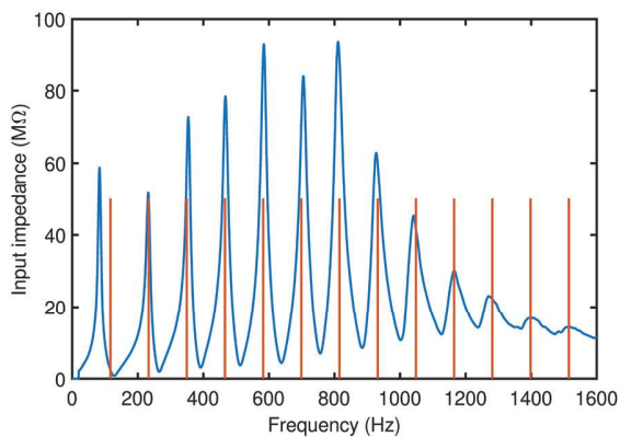
Figure 4. Blue line, input impedance of a B \flat trumpet. Red lines, B \flat harmonic series (integer multiples of 116.5 Hz).
