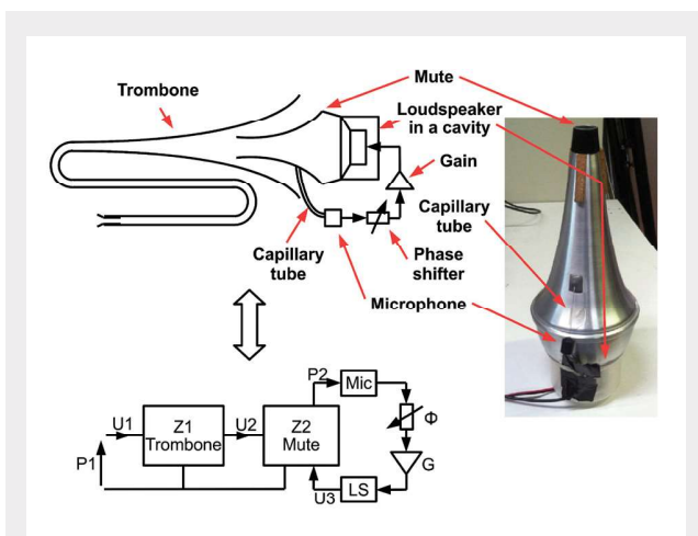
Figure 11. A trombone straight mute with active control system to suppress a parasitic resonance. Top left: schematic diagram of the trombone, mute, and active control apparatus. Bottom left: equivalent circuit of the mute, trombone, and control system. Right: photograph of the active mute. P_1 and U_1 , pressure and volume flow at the trombone input; P_2 and U_2 , pressure measured inside the mute and volume flow at the mute input; Z_1 , trombone input impedance; Z_2 , mute input impedance; U_3 , volume flow generated by the loudspeaker inside the mute. LS, loudspeaker; Mic, microphone. From Meurisse et al., 2015, with permission of the Acoustical Society of America.
