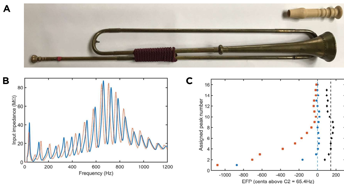
Figure 7. A: natural trumpet (after Hanns Hainlein, 1632) with a modern copy of a baroque mute. B: input impedance curves for a natural trumpet without a mute (blue curve) and with a mute (red curve). C: equivalent fundamental pitch (EFP) for a natural trumpet without a mute (blue circles), with a mute (red squares), and with reassigned peak numbers (black diamonds).
