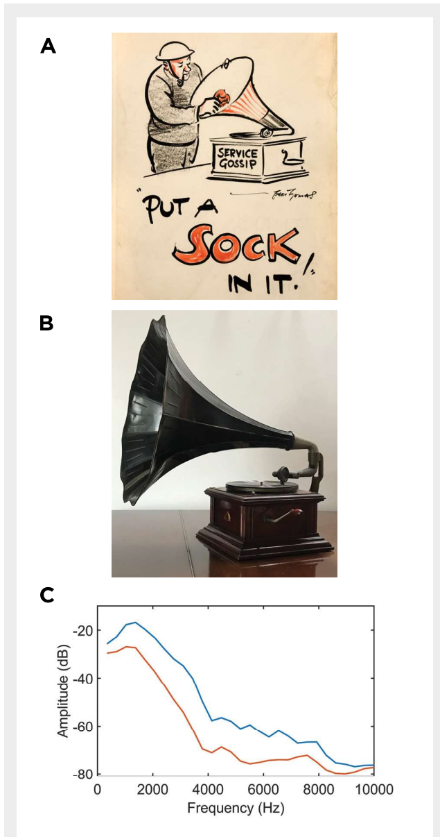
Figure 2. A: British cartoon, c. 1939. Reproduced from the National Archives Image Library, with permission. B: His Masters Voice horn gramophone, early twentieth century. C: long-term average spectra of radiated sound with horn open (blue line) and muted by sock (red line).
