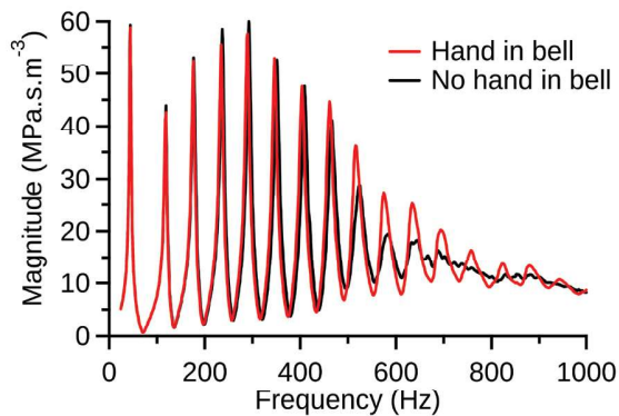
Figure 9. Input impedance curves for F horn with (red) and without (black) hand in bell. From Dell et al., 2010, with permission of the Australian Acoustical Society.
