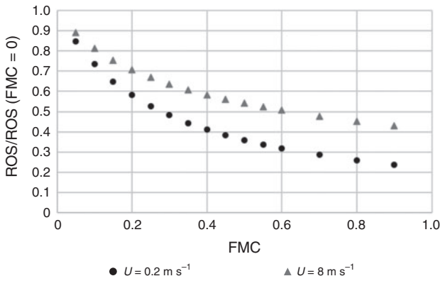
Fig. 4. Relative decay of the rate of spread (ROS; \text{ROS}/\text{ROS}(0\%) ) v. fuel moisture content (FMC).
