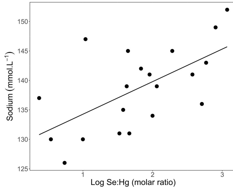
Figure 2. Relation between Se:Hg molar ratio and sodium ( \text{mmol.L}^{-1} , R^2 = 0.378 , p = 0.004 ) in the blood of the Spectacled Caiman ( Caiman crocodilus ) from French Guiana.
