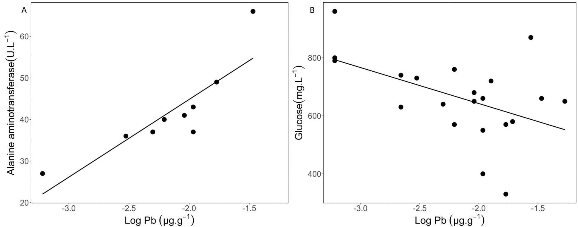
Figure 3. Relation between Pb concentration (Log \mu\text{g.g}^{-1} dw) and (A) Alanine aminotransferase (U.L ^{-1} , R^2 = 0.740 , p = 0.003 ) and (B) Glucose (mg.L ^{-1} , R^2 = 0.239 , p = 0.025 ) in the blood of the Spectacled Caiman ( Caiman crocodilus ) from French Guiana.
