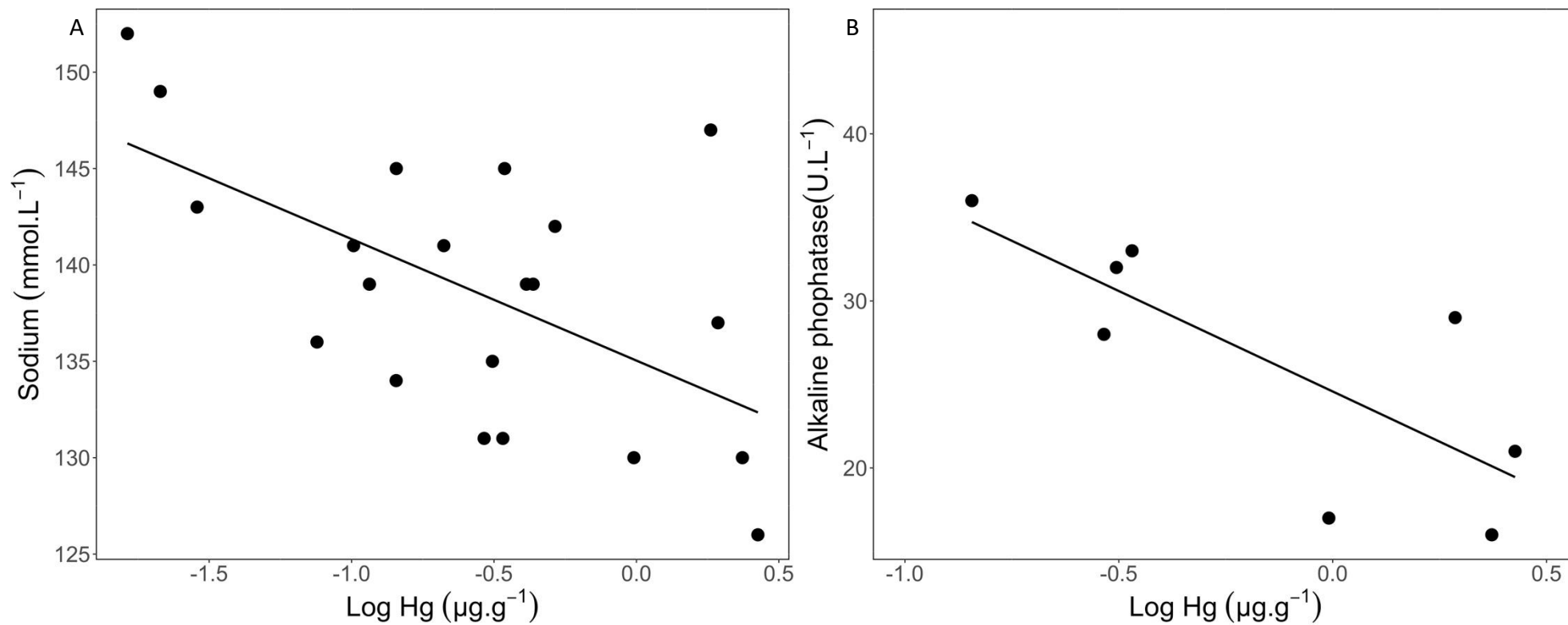
Figure 1. Relation between Hg concentration (Log \mu\text{g.g}^{-1} dw) and (A) sodium (mmol.L -1 , R^2 = 0.345 , p = 0.005 ) and (B) alkaline phosphatase (U.L -1 , R^2 = 0.601 , p = 0.024 ) in the blood of the Spectacled Caiman ( Caiman crocodilus ) from French Guiana.
