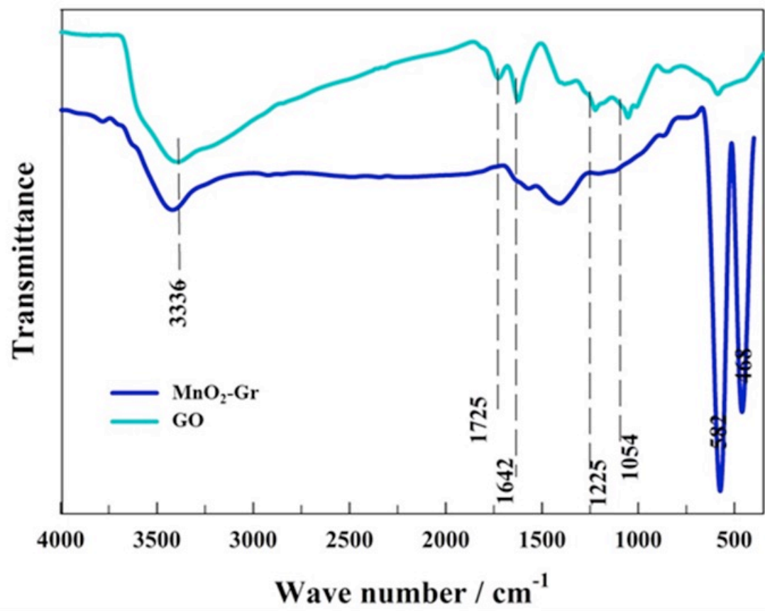
Fig. S1. FTIR spectra of GO and MnO 2 -rGO
