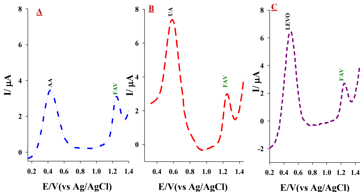
Figure 7. SWVs using a MnO 2 -rGO/SPE in a pH 7.0 B-R buffer containing 5.0 \times 10^{-5} M FAV, 5.0 \times 10^{-3} M AA, UA and LEVO, respectively, for each at scan rate: 0.1 \text{ V s}^{-1} , P_H = 0.25 \text{ V} , P_W = 0.50 \text{ V} , S_H = 0.02 \text{ V} .
