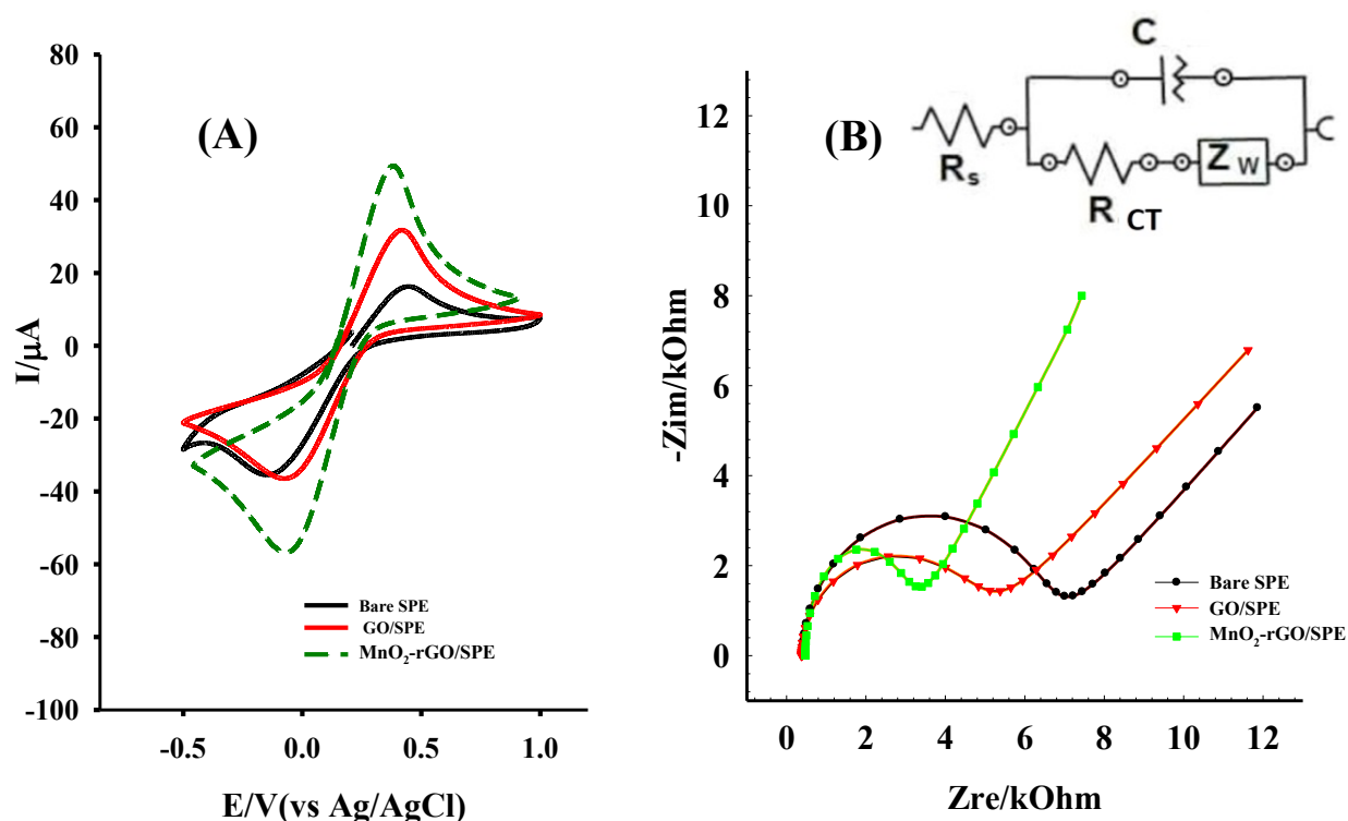
Figure 2. (A) The recorded CV curves at scan rate ( v ) of 0.1 \text{ V s}^{-1} in 5.0 \text{ mM K}_3\text{Fe(CN)}_6 (1:1) in 0.1 \text{ M KCl} solution at SPE, GO/SPE, and \text{MnO}_2\text{-rGO/SPE} electrodes, (B) the electrochemical impedance of each electrode.
