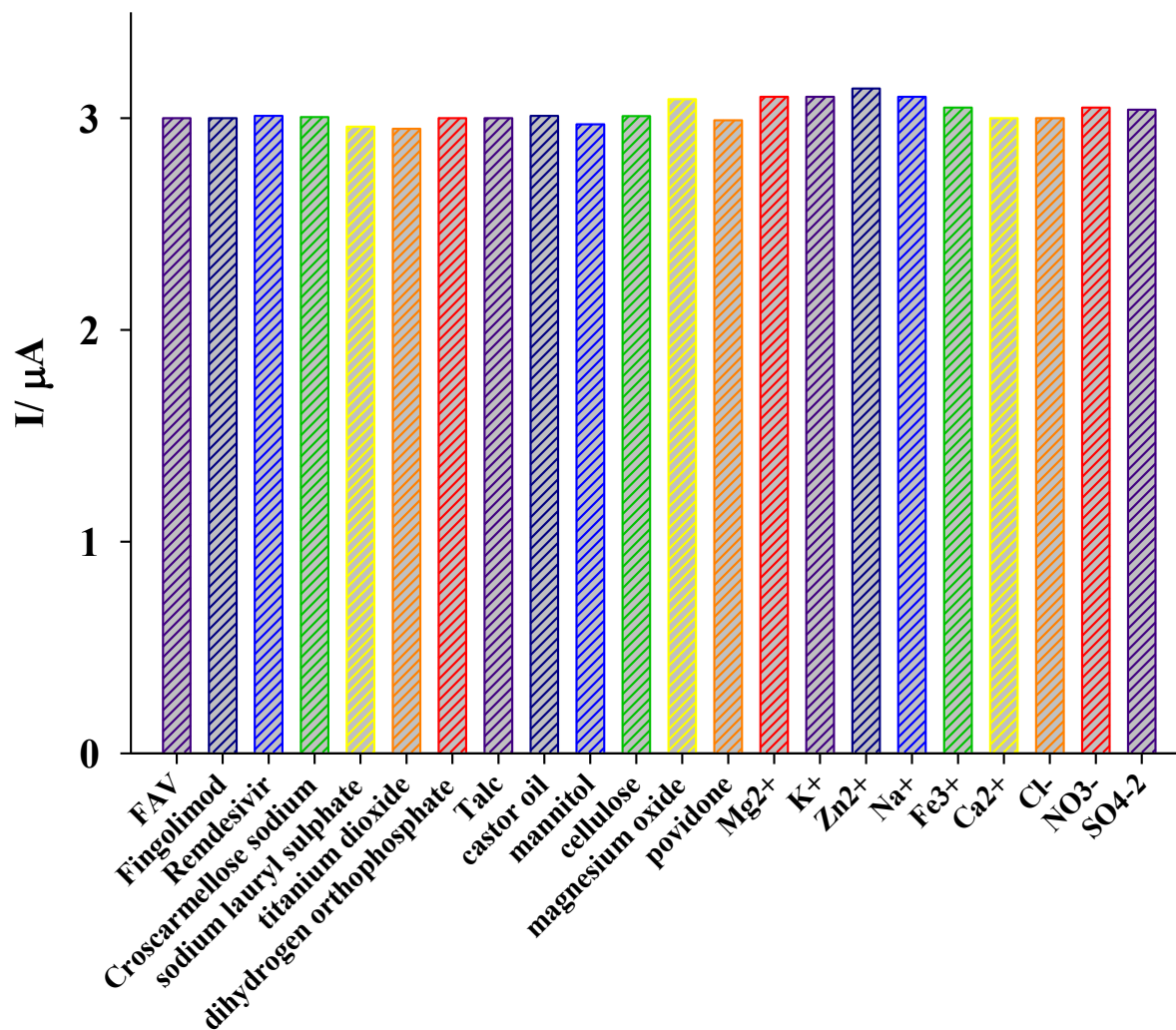
Figure S3. Effect of different interfering materials and ions 1.0 \times 10^{-5} M FAV in a pH 7.0 B.R. buffer (0.04 M) solution.
