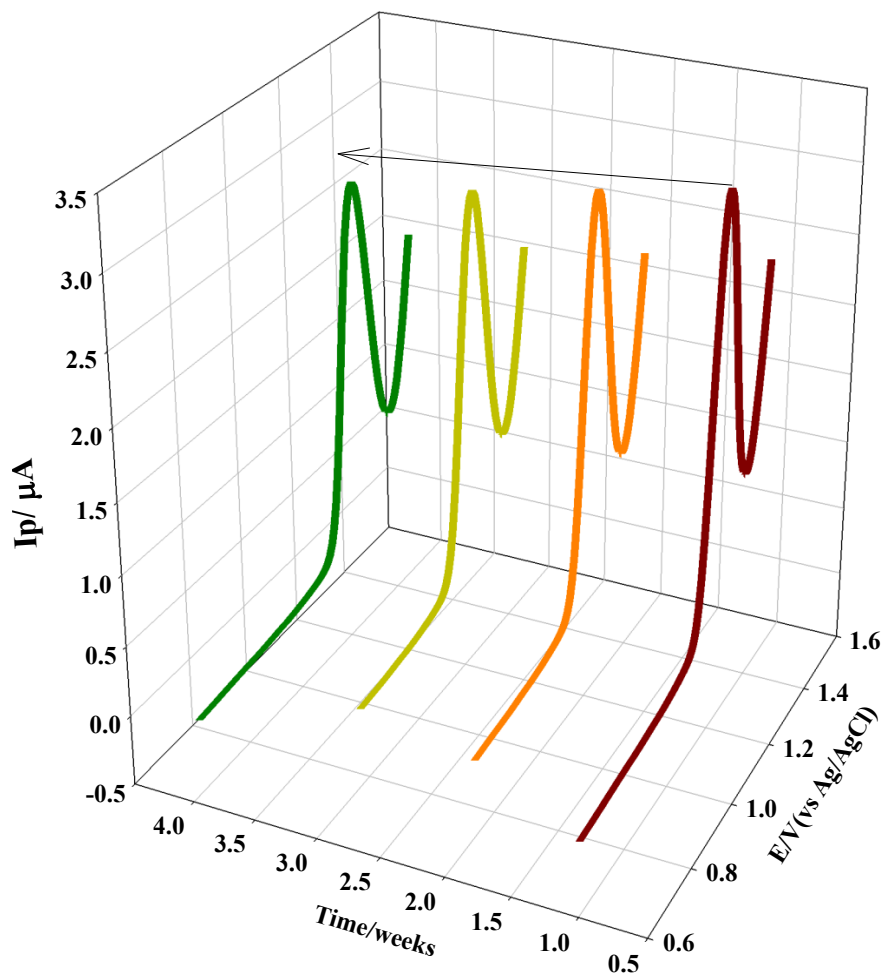
Figure S2. SWVs voltamograms of 1.0 \times 10^{-5} M FAV using MnO_2 -rGO/SPE after 1- 4 weeks storage in B.R. buffer solution (pH= 7.0).
