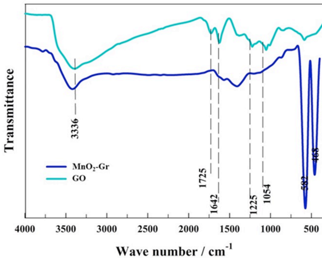
Fig. S1. FTIR spectra of GO and \text{MnO}_2\text{-rGO}
