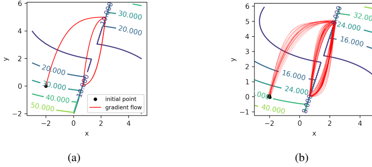
Figure 2: (a) Gradient flow for all implementations. (b) Gradient flows for 20 perturbed experiments.
