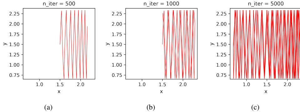
Figure 5: Gradient path after (a) 500, (b) 1000 and (c) 5000 iterations.
