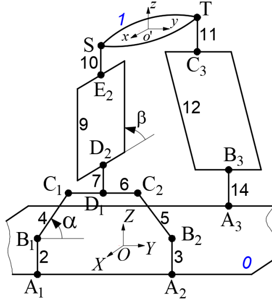
Figure 2. Kinematic modelling of the TPM
