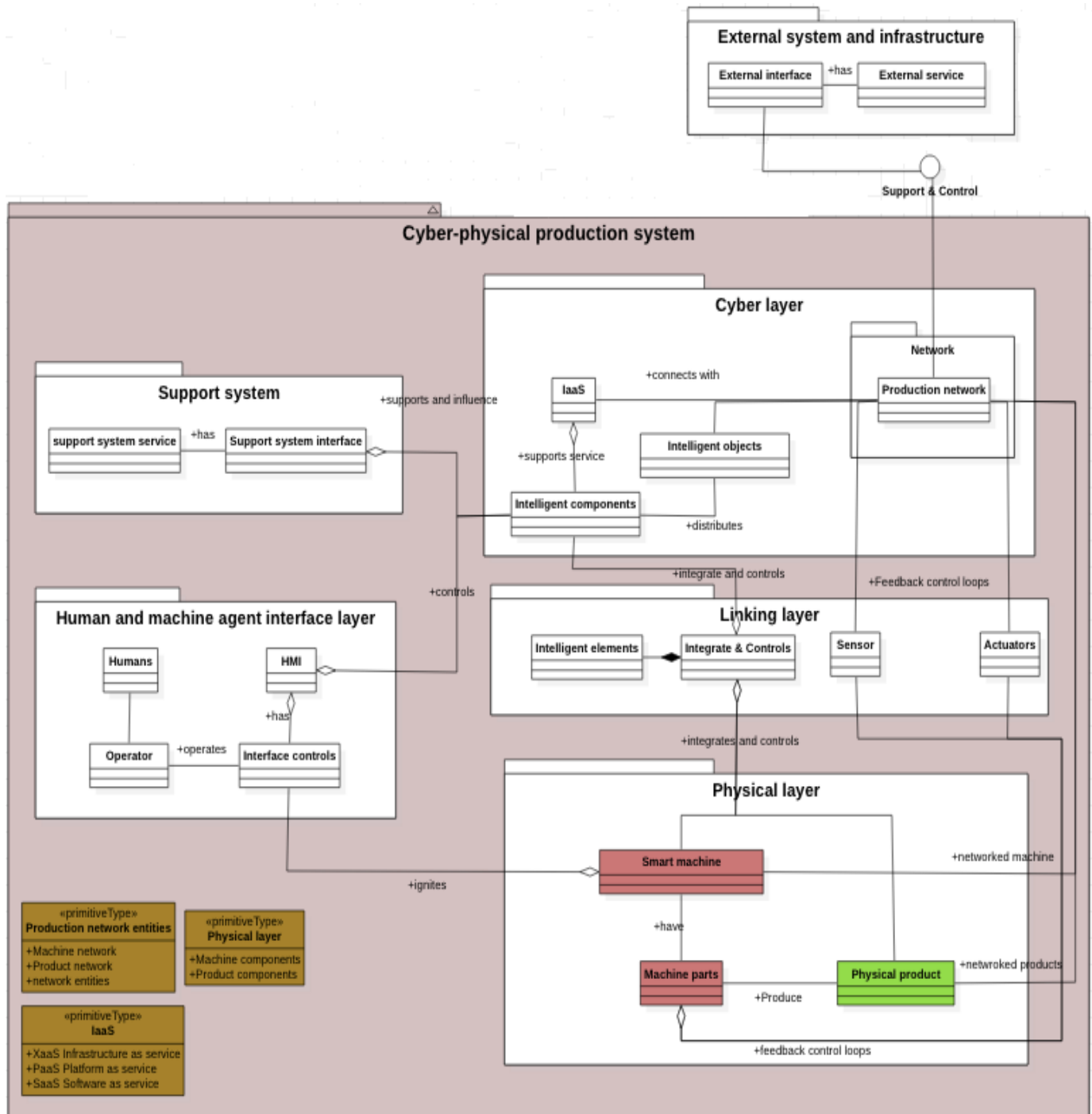
Fig.2. Proposed Generic Semantic model for CPPS
