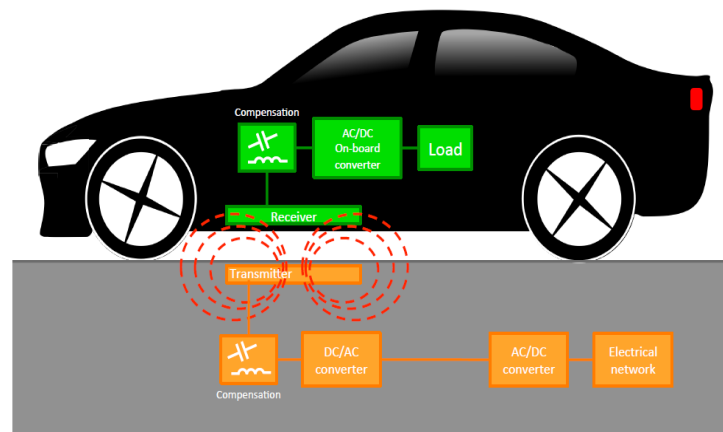
Figure 1. A static inductive power transfer system for electric vehicles [21].
