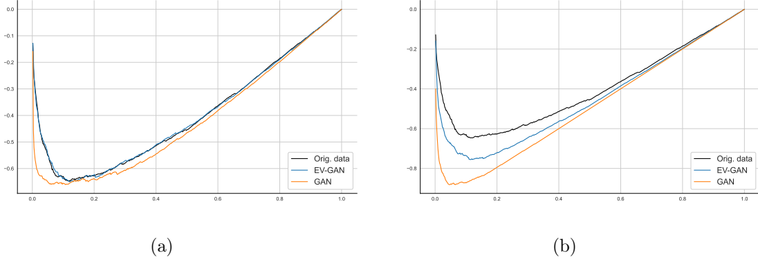
Figure 8: Estimated \lambda(\cdot) functions associated with the World market zone ( d = 6 ). Black: original real data, blue: data generated with EV-GAN model, orange: data generated with classic GAN model. (a) AKE criterion, (b) SSLE(0.95) criterion.
