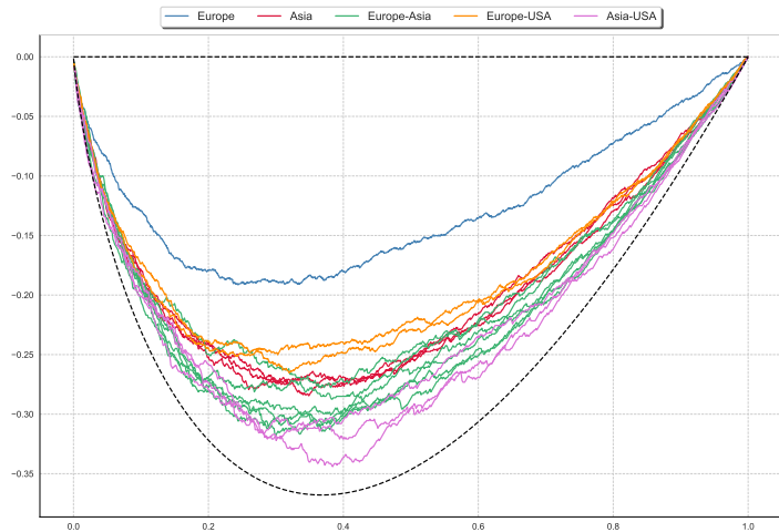
(g) Estimated \lambda(\cdot) functions
