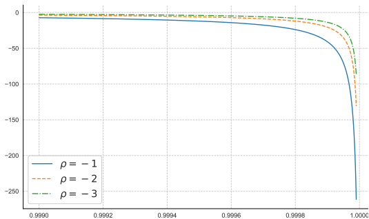
(a) TIF with \gamma = 1/2 and \rho \in \{-3, -2, -1\}
