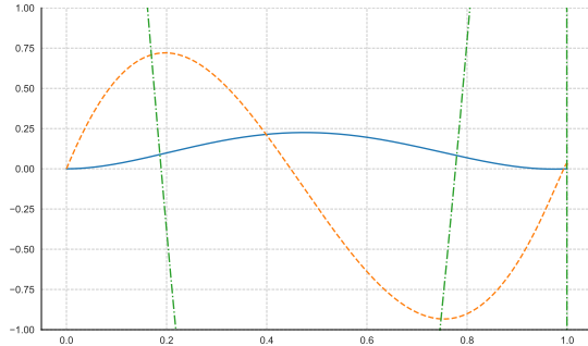
(b) CTIF with \gamma = 1/2 and \rho = -1
