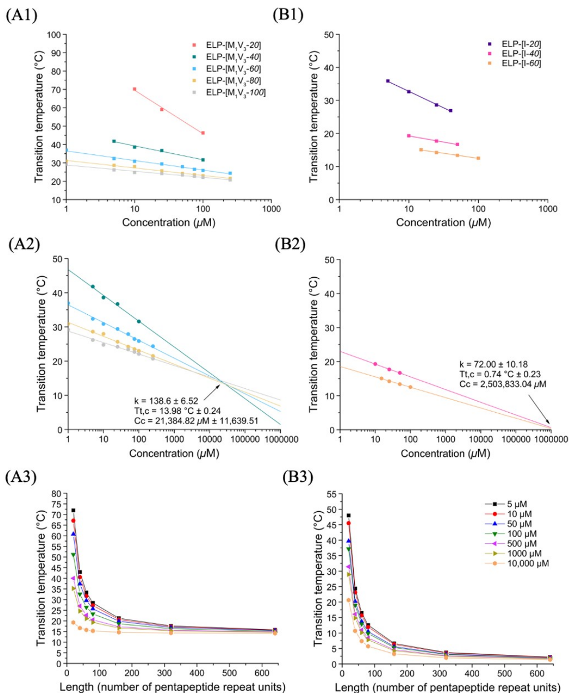
Figure 2. Thermal study of monoblock ELPs in PBS. (A) ELP-[M 1 V 3 -i]. (B) ELP-[I-i]. (1) T_t values as function of sample concentration and log fitted. (2) Simulation of T_t values in a larger concentration range from 1 to 1,000,000 \mu\text{M} allowing T_{t,c} and C_c determination. (3) T_t values at different L , j = length ( L ).
