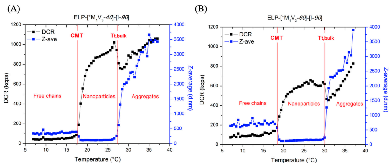
Figure 8. DLS measurement of 10 \mu M (A) ELP-[ M_1V_3-40 ]-[I-90] and (B) ELP-[ M_1V_3-60 ]-[I-90] in PBS on a thermal ramp 7–40 °C (DCR: Derived Count Rate, the parameter representative of the scattering intensity. Z-ave: the Z-average value, i.e., the intensity-weighted mean hydrodynamic size of the particles ensemble).
