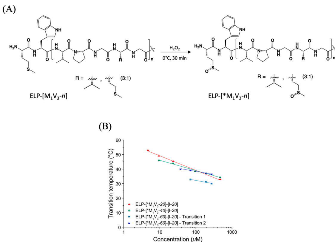
Figure 4. (A) Chemical structure of oxidized ELP. (B) Tt values of ELP-[*M 1 V 3 - i ]-[I-20] ( i = 20, 40, 60) in ultrapure water as function of sample concentration and log fitted.
