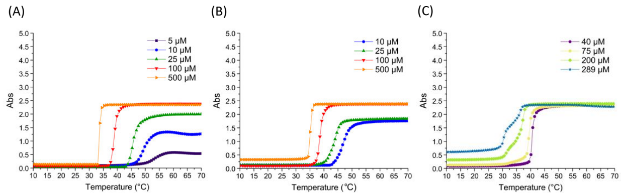
Figure S12. Turbidity assays at 350 nm with a rate of 1°C/min of (A, B, C) ELP-[*M 1 V 3 - i ]-[I-20] ( i = 20, 40, 60 respectively) in ultrapure water.
