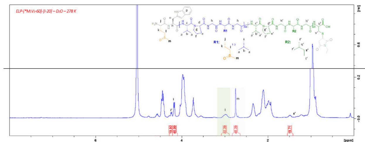
Figure S8. NMR spectra in D 2 O of (A) ELP-[ * M 1 V 3 -20]-[I-20] (B) ELP-[ * M 1 V 3 -40]-[I-20] (C) ELP-[M 1 V 3 -60]-[I-20]. A part of the spectra was removed for a better view on interesting peaks. Green and gray boxes highlight resonances for CH 2 and CH 3 bonded to sulfur of the methionine, respectively.
