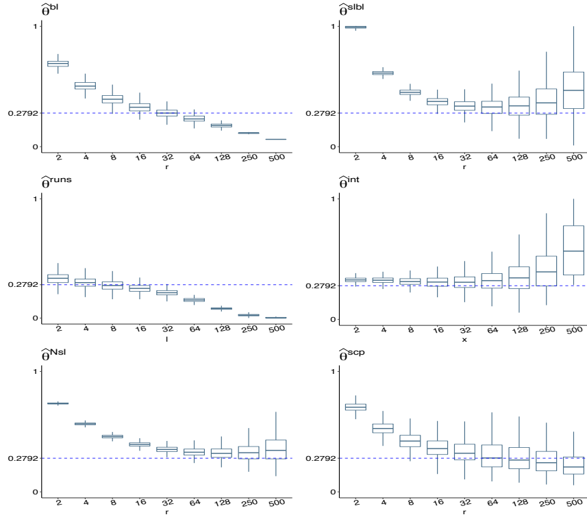
Figure 5.2. Boxplots based on 1 000 simulations for the estimation of \theta_X \approx 0.2792 for the solution to a stochastic recurrence equation.
