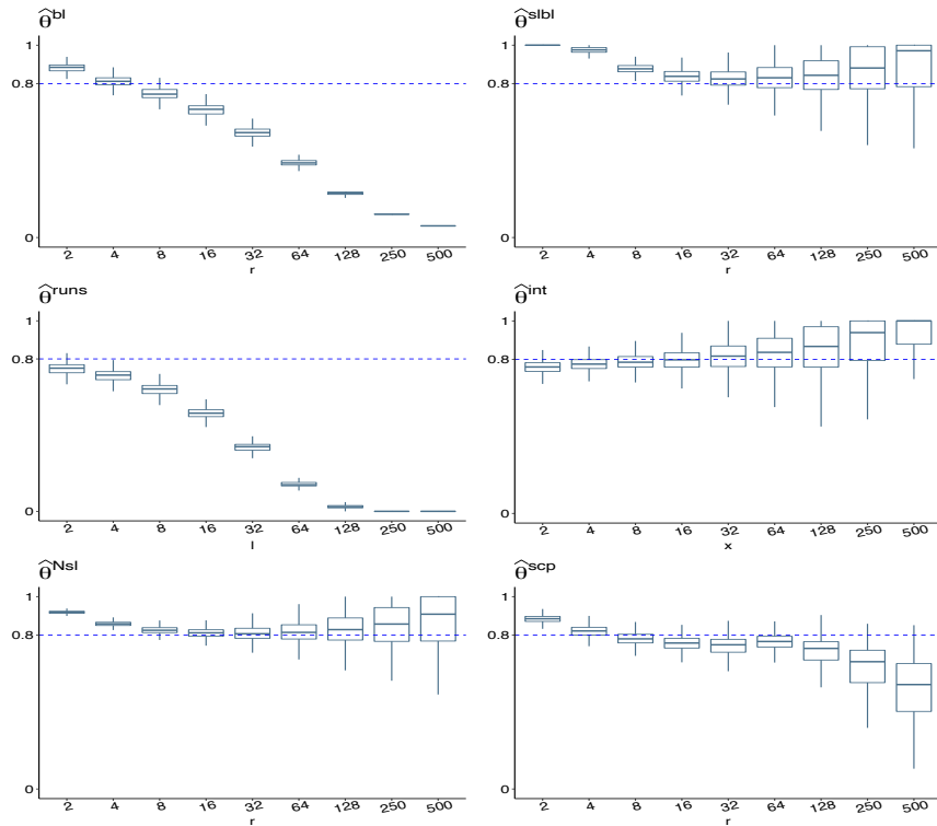
Figure 5.1. Boxplots based on 1000 simulations for the estimation of \theta_{|X|} = 0.8 in the AR(1) model with \varphi = 0.2 and iid student(1) noise.
