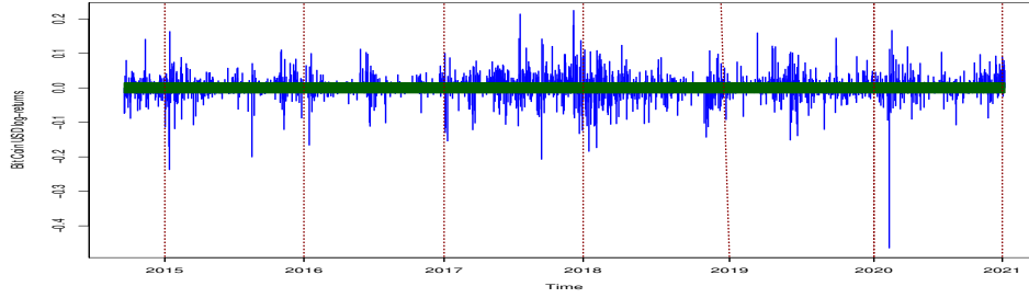
Figure 2.2. The daily log-return series of the Bit Coin USD stock prices from 17 September 2014 until 8 January 2021. We only show the returns below -0.04 or above 0.04 which we interpret as extreme values. These limits roughly correspond to the 10% and 90% quantiles of the data. The extremes typically appear in clusters.
