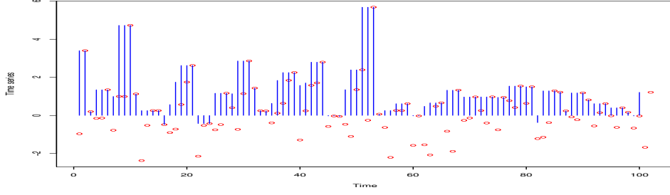
Figure 2.1. Visualization of the max-moving average X_t = \max(Z_t, Z_{t+1}, Z_{t+2}) , t = 1, \dots, 100 , (blue) for iid student noise Z_t , t = 1, \dots, 102 , with \alpha = 4 degrees of freedom (red dots). The values of X_t typically appear in clusters of size 3. The process (|X_t|) has extremal index \theta_{|X|} = 1/3 .
