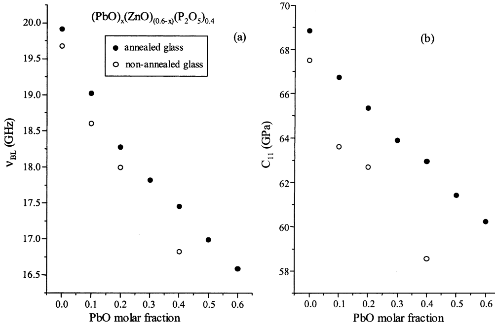
Fig. 2. Longitudinal Brillouin shift \nu_{BL} (a) and elastic constant C_{11} (b) in (\text{PbO})_x(\text{ZnO})_{(0.6-x)}(\text{P}_2\text{O}_5)_{0.4} glasses versus composition.
