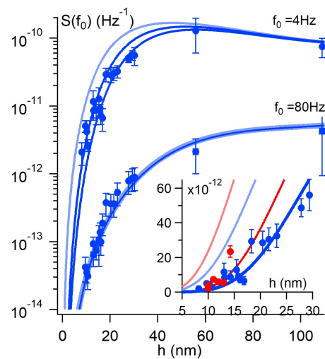
FIG. 4. Fluctuation spectra (in logarithmic scale) of oil films (viscosity 19 mPa·s) at 4 Hz and 80 Hz, as a function of film thickness. The full lines correspond to theoretical predictions without (lighter lines) and with (darker lines) intermolecular forces, with |A| = 10^{-19} J and |A| = 2 \times 10^{-19} J. Inset: Fluctuation spectra (in linear scale) at 4 Hz of the two oil films with viscosity 19 mPa·s (blue circles, same data as main figure) and 9.3 mPa·s (red circles). Vertical error bars correspond to the statistical uncertainty. Horizontal error bars are too small to appear.
