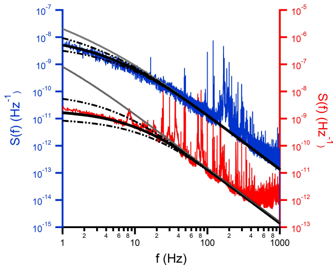
FIG. 3. Fluctuation spectra of oil films of thickness 30.3 nm (viscosity 19 mPa·s, blue, left axis) and 12.9 nm (viscosity 9.3 mPa·s, red, right axis). Spurious peaks result from parasitic noise either of mechanical or electromagnetic origin. For each spectrum, the full lines represent the theoretical spectra without (grey lines) and with (black lines) intermolecular forces effects. Dash-dotted lines correspond to spectra computed with Hamaker constants differing by \pm 50\% .
