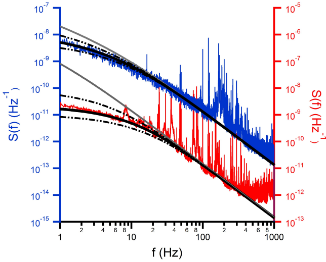
FIG. 3. Fluctuation spectra of oil films of thickness 30.3 nm (viscosity 19 mPa·s, blue, left axis) and 12.9 nm (viscosity 9.3 mPa·s, red, right axis). Spurious peaks result from parasitic noise either of mechanical or electromagnetic origin. For each spectrum, the full lines represent the theoretical spectra without (grey lines) and with (black lines) intermolecular forces effects. Dash-dotted lines correspond to spectra computed with Hamaker constants differing by \pm 50\% .
