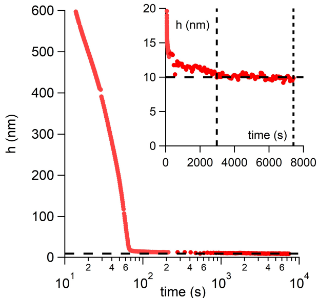
FIG. 2. Thickness of film of a silicone oil (viscosity 9.3 mPa·s) under the laser beam as a function of time. Insert shows details of the plateau corresponding to h_0 = 10.0 \pm 0.3 nm.
