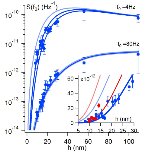
FIG. 4. Fluctuation spectra (in logarithmic scale) of oil films (viscosity 19 mPa·s) at 4 Hz and 80 Hz, as a function of film thickness. The full lines correspond to theoretical predictions without (lighter lines) and with (darker lines) intermolecular forces, with |A| = 10^{-19} J and |A| = 2 \times 10^{-19} J. Inset: Fluctuation spectra (in linear scale) at 4 Hz of the two oil films with viscosity 19 mPa·s (blue circles, same data as main figure) and 9.3 mPa·s (red circles). Vertical error bars correspond to the statistical uncertainty. Horizontal error bars are too small to appear.
