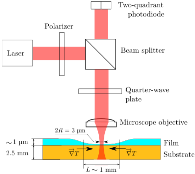
FIG. 1. Schematized experimental set-up (not to scale). The laser is focused on the liquid film spread on a colored glass substrate. Light absorption by the substrate creates a thermal gradient in the liquid layer over the lengthscale L , which also define the extension of the film thinning.
