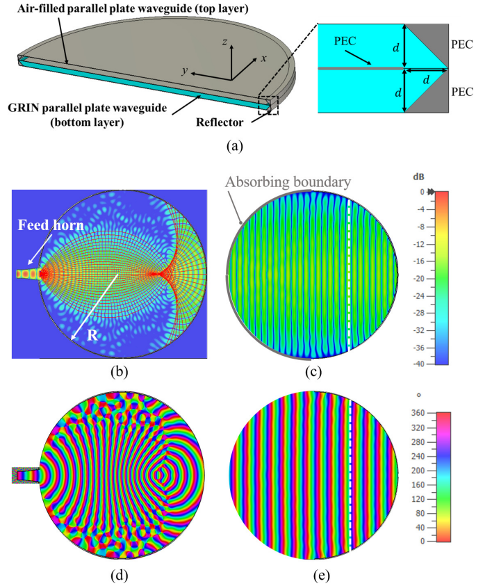
Fig. 4. (a) Perspective view of simulated RLL cutted in the yz plane, and inset with detail of the corner reflector. Real part of the vertical component of the electric field in logarithmic scale for (b) the bottom and (c) the top PPWs. Phase distribution in degrees for (d) the bottom and (e) the top PPWs.
