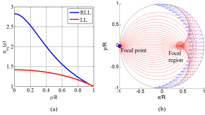
Fig. 3. (a) Radial profile of the refractive index of the RLL (blue line) and of the equivalent Luneburg Lens (red line) for n_0 = n_1 = 1 . (b) Ray-paths of the RLL (red lines) and direction of reflected rays in upper PPW (blue arrows).
