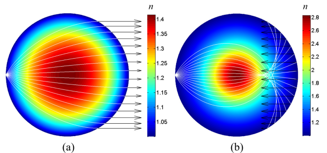
Fig. 1. Comparison between (a) Luneburg Lens and (b) Reflecting Luneburg Lens (RLL). In the RLL, the rays emerging from a point at the periphery undergo longer paths and, after reflecting at the boundary, they are coupled to an upper uniform guiding layer, where they form a plane wave.
