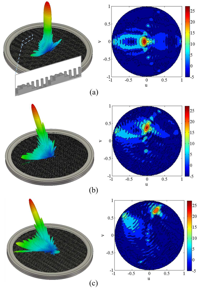
Fig. 6. 3D view of the radiated beam (left column) and u-v color maps (right column) showing the directivity in dBi when the angle of the excited horn in Fig. 5 with the x -axis is (a) 0^\circ , (b) 20^\circ and (c) 40^\circ .
