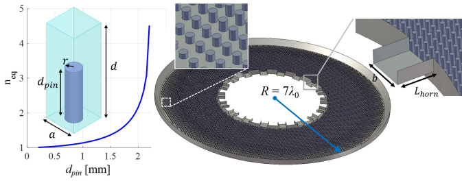
Fig. 5. Left: Mapping between the height of a metallic pin and equivalent refractive index where r = 0.3 mm, a = 1.25 mm, and d = 3.75 mm for an operating frequency of 30 GHz. Right: Bottom PPW for the multibeam RLL beamformer implemented by a bed of nails, the radius of the structure is R = 7\lambda_0 , where \lambda_0 is the free-space wavelength at 30 GHz.
