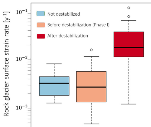
Fig. 6 Rock glacier surface strain rates measured at the local sites. The strain rate is measured as a variation of displacement rates ( \text{my}^{-1} ) over the distance between the two points projected on the central flow axis. This is done for each period where displacement rate pairs were available on the orthoimages. Low strain rate values in destabilised rock glaciers refer to the deceleration of the destabilised area (Phase IV—Fig. 1). The boxplot respect the standardized sizes: the interquartile (IQR) range groups observations from the 25th (Q1) to 75th (Q3) percentile, while the whiskers represent the maximum ( Q3 + 1.5 \times \text{IQR} ) and minimum ( Q1 - 1.5 \times \text{IQR} ).
