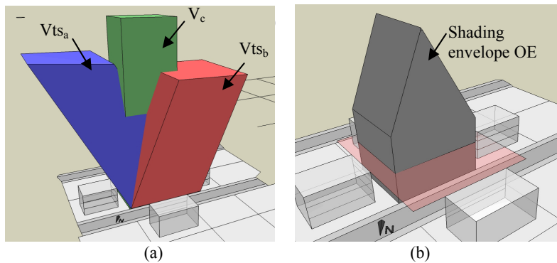
Fig. 5 (a) Volumes used in the construction of the Shading Envelope: V_{tsa} (according to the sun direction at 10h), V_{tsb} (according to the sun direction at 14h) and V_c (from parcel base); (b) Shading Envelope EO = V_{tsa} \cap V_{tsb} \cap V_c .
