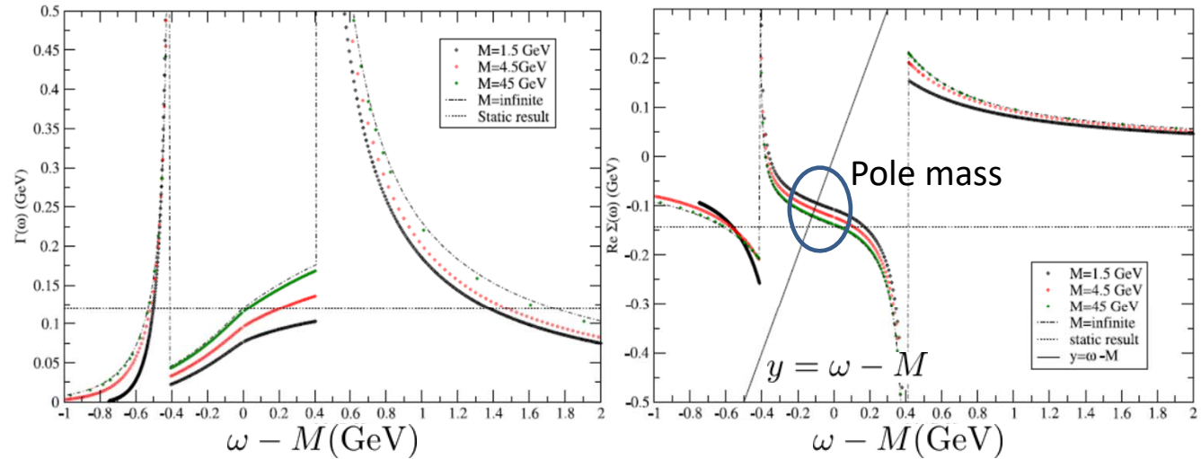
Fig. 6. (Color on-line.) Imaginary part (left) and real part (right) of the self-energy \Sigma . The horizontal lines, labelled “static limit”, indicate the values of \Gamma(M \rightarrow \infty) and \text{Re } \Sigma(M \rightarrow \infty) . With the parameters \alpha = 0.4 and T = 300 MeV, these are respectively 120 MeV and -143 MeV. Within the gap \pm\omega_{pl} , \Gamma is an increasing function of M , while \text{Re } \Sigma is a decreasing function of M . Both functions nearly reach the infinite mass limit when M = 45 GeV.
