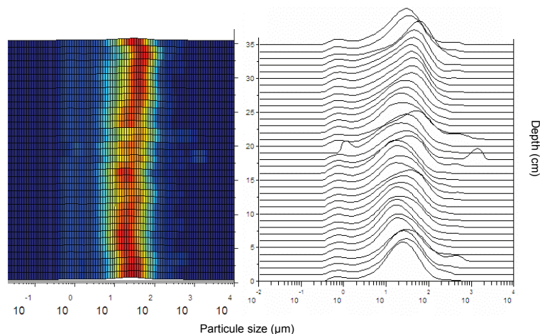
Figure 4: Particle Size Distribution of core LDB06-L2 (taken near the outlet of the Leyse River)
