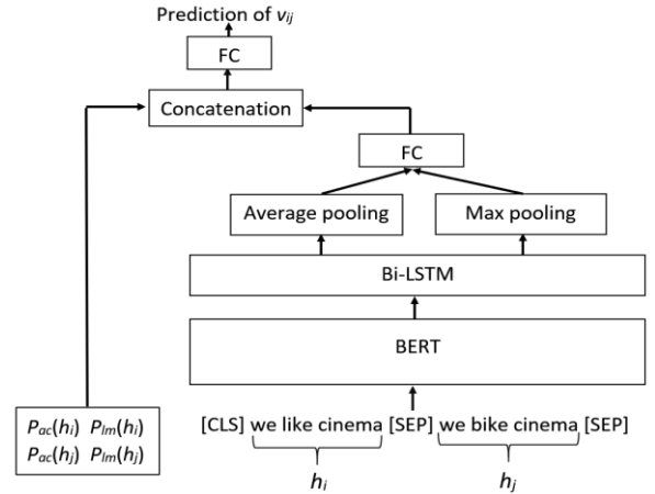
Figure 1: Proposed BERT alsem rescoring model.
