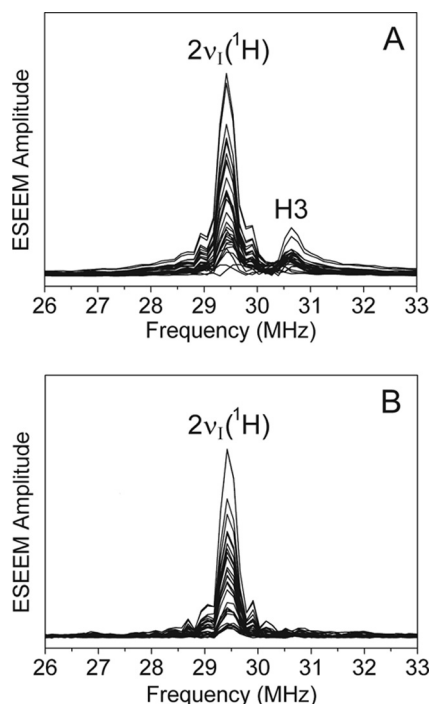
FIGURE 3. Stacked presentations of the two-dimensional set of the four-pulse ESEEM spectra of MSQ D in 1 H 2 O (A) and 2 H 2 O (B). The spectra show modulus Fourier transforms along the time T/2 axis (1024 points with a 4 ns step) at 30 different times \tau . The initial \tau is 96 ns and was increased by 8 ns in successive traces. The microwave frequency was 9.6912 GHz (A) and 9.6898 GHz, and the magnetic field was 345.2 mT (A) and 345.4 mT (B).
