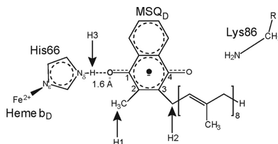
FIGURE 5. Working model of MSQ D binding mode in E. coli NarGHI based on our spectroscopic work. Strongly asymmetric binding of MSQ D occurs via a short in-plane H-bond to the N δ of His-66, whereas Lys-86 does not appear to be a direct H-bond donor to the radical in the semiquinone state (13). The MSQ D O4 oxygen is deprotonated. The protons H1, H2, and H3 discussed under "Results" are indicated by arrows. r = \text{NHCCO}(\text{CH}_2)_3 .
