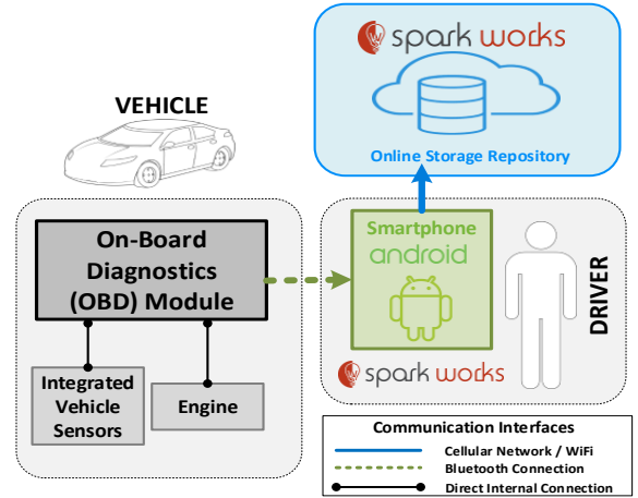
Fig. 3: System Architecture
