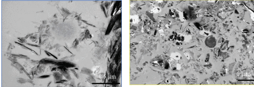
Figure 2 : TEM observation of particles entering in the infiltration pond of Chevéré
