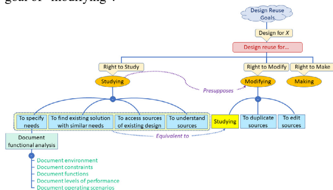
Fig. 4. Illustration of how design guidelines relate to design reuse goals.
