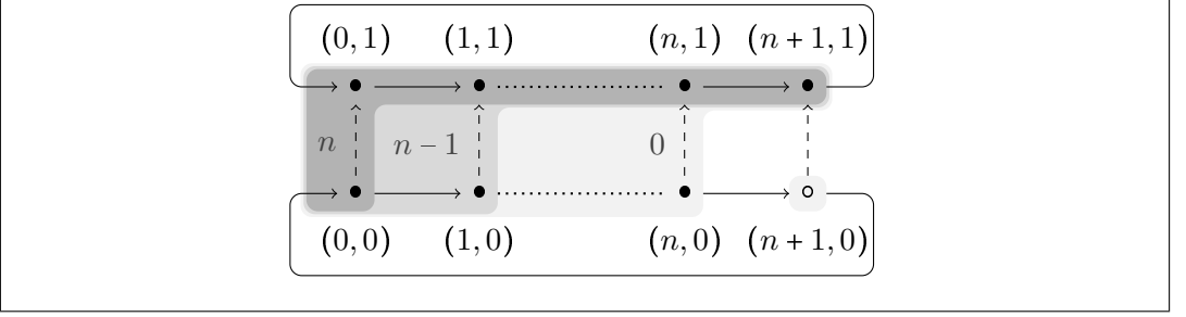
Figure 1: The here-and-there model \mathcal{H}_n . Black dots satisfy the atom p , white dots do not; all other atoms are false everywhere. Dashed lines indicate \preceq and solid lines indicate S . The \sim_i -equivalence classes are shown as grey regions.
