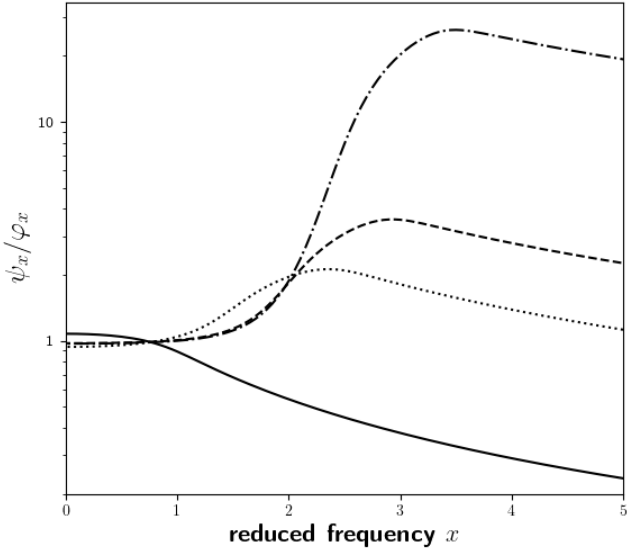
Fig. 3. Ratios \psi_x/\varphi_x as a function of the reduced frequency x , for the different radiation field profiles displayed in Fig. 1, using also the same linestyle convention. We observe here, for the case of coherent scattering in the atom’s frame, similar tendencies as the ones displayed in Fig. 2 for the ratios between VDFs.
