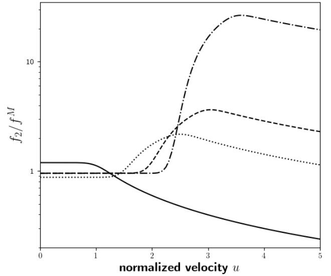
Fig. 2. Ratios f_2/f^M as a function of the normalized velocity u , for different radiation field profiles, and for \varepsilon = 0 and \zeta = 0 . The same linestyle convention as in Fig. 1 was adopted. The magnitude of these departures from a Maxwellian velocity distribution depends on both (i) the distance of the peaks of I vs. line center, and (ii) the amount of its central reversal characterized by I_{max}/I(0) .
