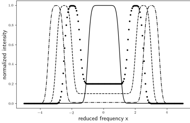
Fig. 1. Isotropic and normalized intensity profiles I vs. the reduced frequency x , used for the evaluation of departures from the equilibrium velocity distribution for the VDF of these excited atoms, f_2 . We adopted different values for (i) the location of the (symmetric) peaks, and (ii) of the central reversal of each profile. These variations can also mimic some resonance lines observations that may form under different astrophysical conditions.
