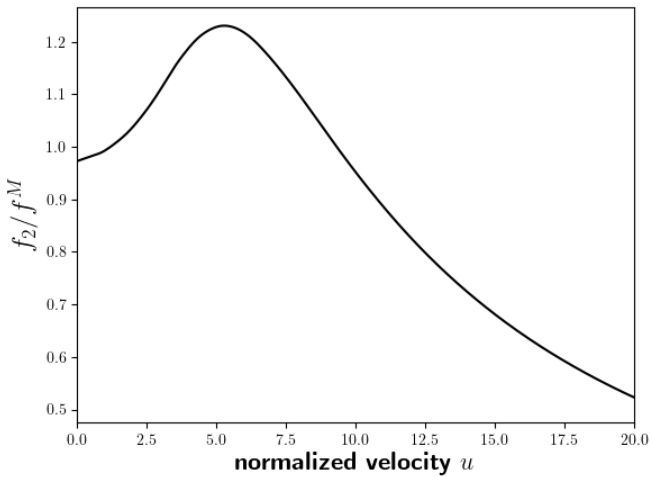
Fig. 4. Ratio f_2/f^M vs. the normalized velocity u for \varepsilon = 10^{-7} ( \zeta = 0 ), and a realistic H I Ly \alpha illumination profile as observed by SoHO/Sumer. The peak of the line profile is located at x \sim 5 , and the central self-reversal is about 0.7 for this resonance line (see Fig. 5 of Gunár et al. 2020).
