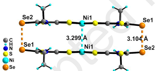
Figure 3. Detail of one dimer in the structure of [Ni(Et-thiazSedt) 2 ].
