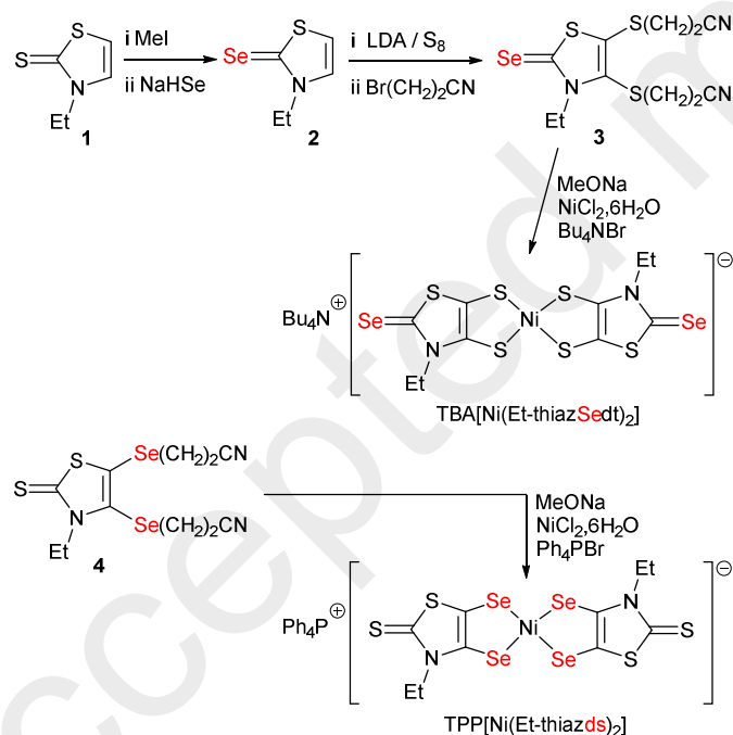
Scheme 1. Syntheses of the anionic complexes [\text{Ni}(\text{Et-thiazSedt})_2]^{-} and [\text{Ni}(\text{Et-thiazds})_2]^{-} .
