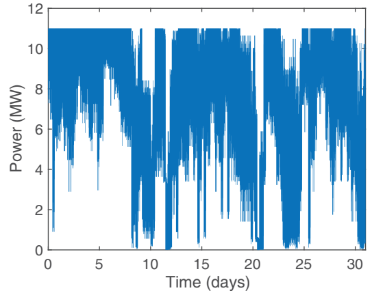
FIGURE 3 Power profile of the wave farm (1st January–31st January, 2015) used for the comparative analysis of the electrothermal models
