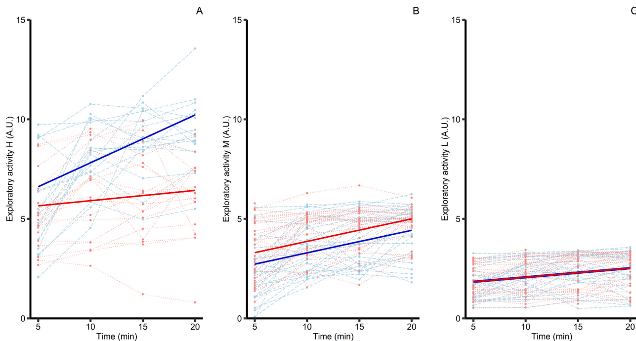
Fig. 2. Exploratory pattern over time in the open field test according to the dose treatment exposure. Blue: control fish; red: exposed fish; Solid lines: predicted models; dashed lines: individual changes in exploratory activity of control fish; dotted lines: individual changes in exploratory activity of exposed fish. A) H: high dose. B) M: medium dose. C) L: low dose. (For interpretation of the references to colour in this figure legend, the reader is referred to the web version of this article.)
