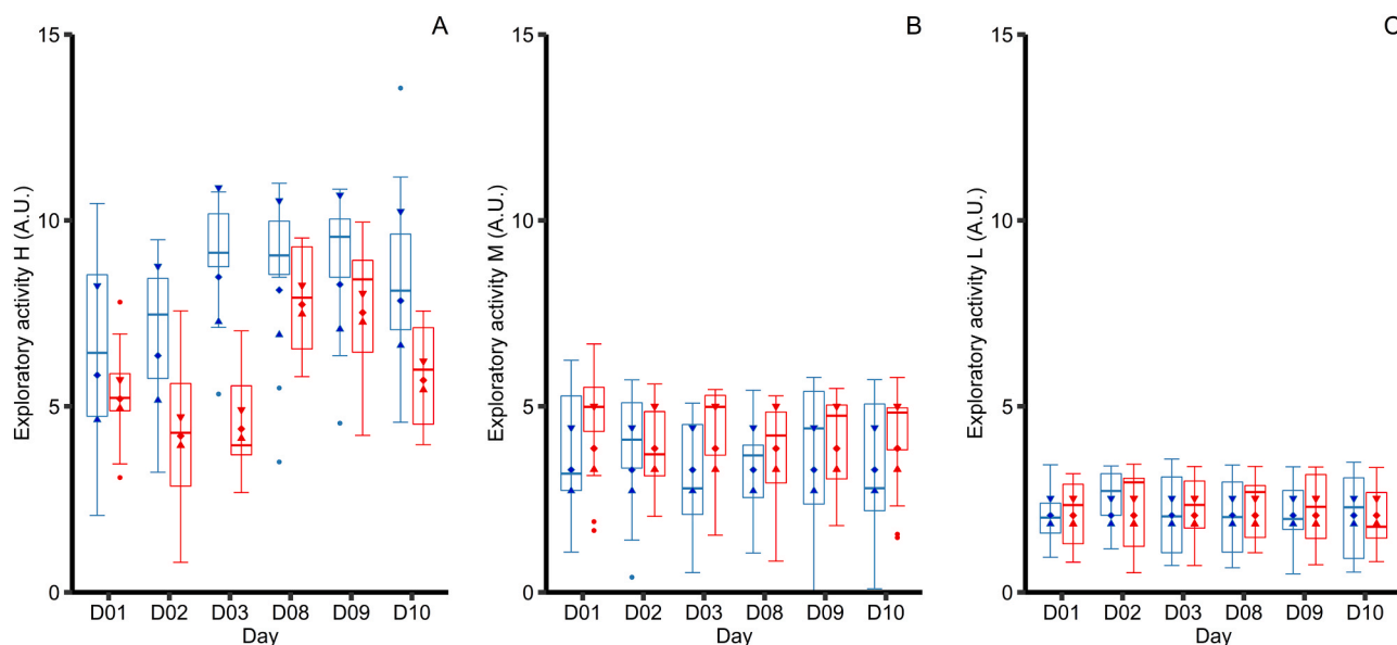
Fig. 3. Exploratory activity over post-exposure days 1, 2, 3, 8, 9 and 10 according to the dose treatment exposure. Blue: control fish; red: exposed fish; \Delta : predicted value after 5 min in the open field test (OFT); \diamond : predicted value after 10 min in the OFT; \nabla : predicted value after 20 min in the OFT. The boundary of the box closest to zero indicates the 25th percentile, a black line within the box marks the median and the boundary of the box farthest from zero indicates the 75th percentile. Whiskers above and below the box indicate the 10th and 90th percentiles. Points above and below the whiskers indicate outliers outside the 10th and 90th percentiles. A) H: high dose. B) M: medium dose. C) L: low dose. (For interpretation of the references to colour in this figure legend, the reader is referred to the web version of this article.)
