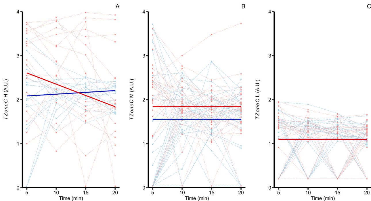
Fig. 4. Time spent in the central zone ( TZoneC ) over the 20 min of the open field test according to the dose treatment exposure. Blue: control fish; red: exposed fish. Solid lines: predicted models; dashed lines: trends of control individuals; dotted lines: trends of exposed individuals. A) H: high dose. B) M: medium dose. C) L: low dose. (For interpretation of the references to colour in this figure legend, the reader is referred to the web version of this article.)
