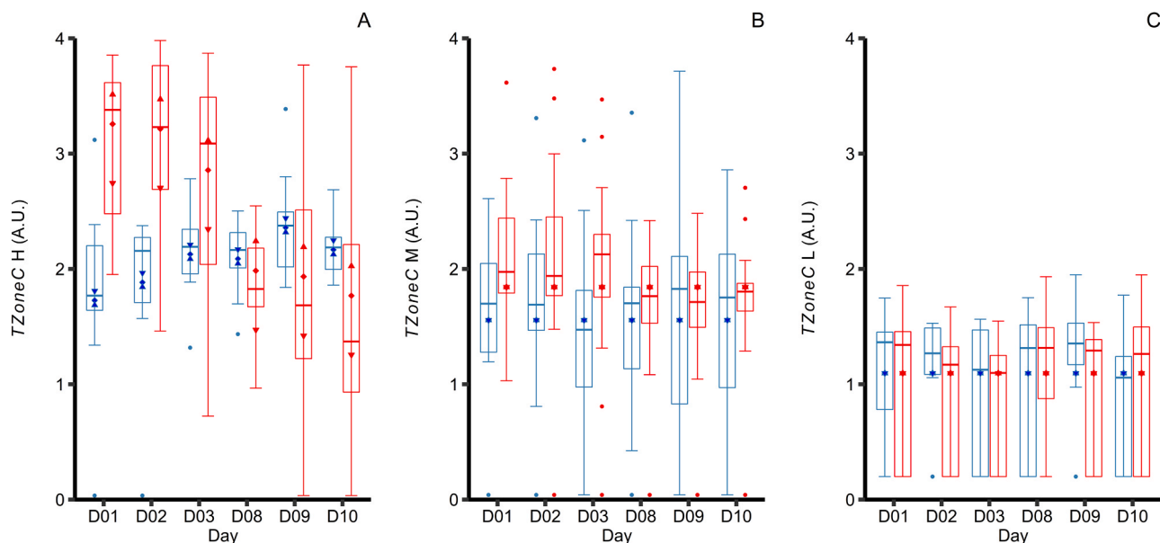
Fig. 5. Time spent in the central zone ( TZoneC ) over the 20 min of the open field test according to the dose treatment exposure. Blue: control fish; red: exposed fish; \Delta : predicted value after 5 min in the open field test (OFT); \diamond : predicted value after 10 min in the OFT; \Delta : predicted value after 20 min in the OFT. The boundary of the box closest to zero indicates the 25th percentile, a black line within the box marks the median and the boundary of the box farthest from zero indicates the 75th percentile. Whiskers above and below the box indicate the 10th and 90th percentiles. Points above and below the whiskers indicate outliers outside the 10th and 90th percentiles. A) H: high dose. B) M: medium dose. C) L: low dose. (For interpretation of the references to colour in this figure legend, the reader is referred to the web version of this article.)
