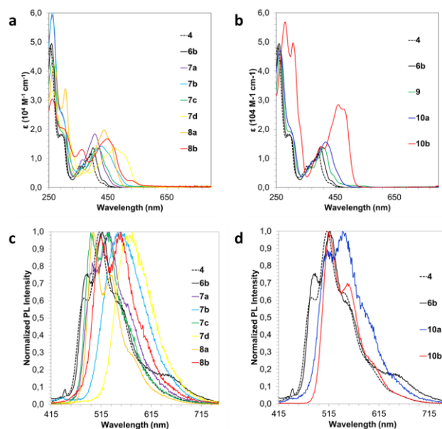
Figure 2. (a-b) UV-vis. absorption and (c-d) fluorescence spectra of compounds 4, 6b, 7a-d, 8a-b, 9 and 10a-b, excited at 400 nm. All measurements were performed in air-equilibrated 10 \mu M chloroform solutions at room temperature.
