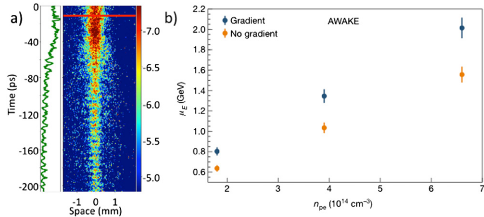
Figure 3. (a) Time-resolved picture of the self-modulated proton bunch (from [7]), (b) energy gain as a function of plasma density without (orange symbols) and with (blue symbols) plasma density gradient (from [23]).
