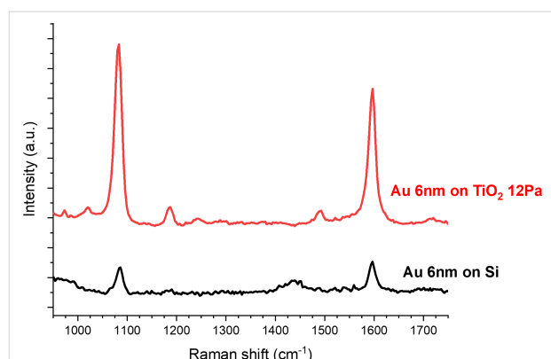
Figure 6: SERS enhancement measured for MBA of the same equivalent thickness of evaporated Au deposited on top of a bare Si(100) substrate (black line) and a nanostructured TiO 2 film (red line).
