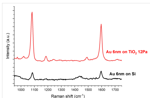
Figure 6: SERS enhancement measured for MBA of the same equivalent thickness of evaporated Au deposited on top of a bare Si(100) substrate (black line) and a nanostructured TiO 2 film (red line).
