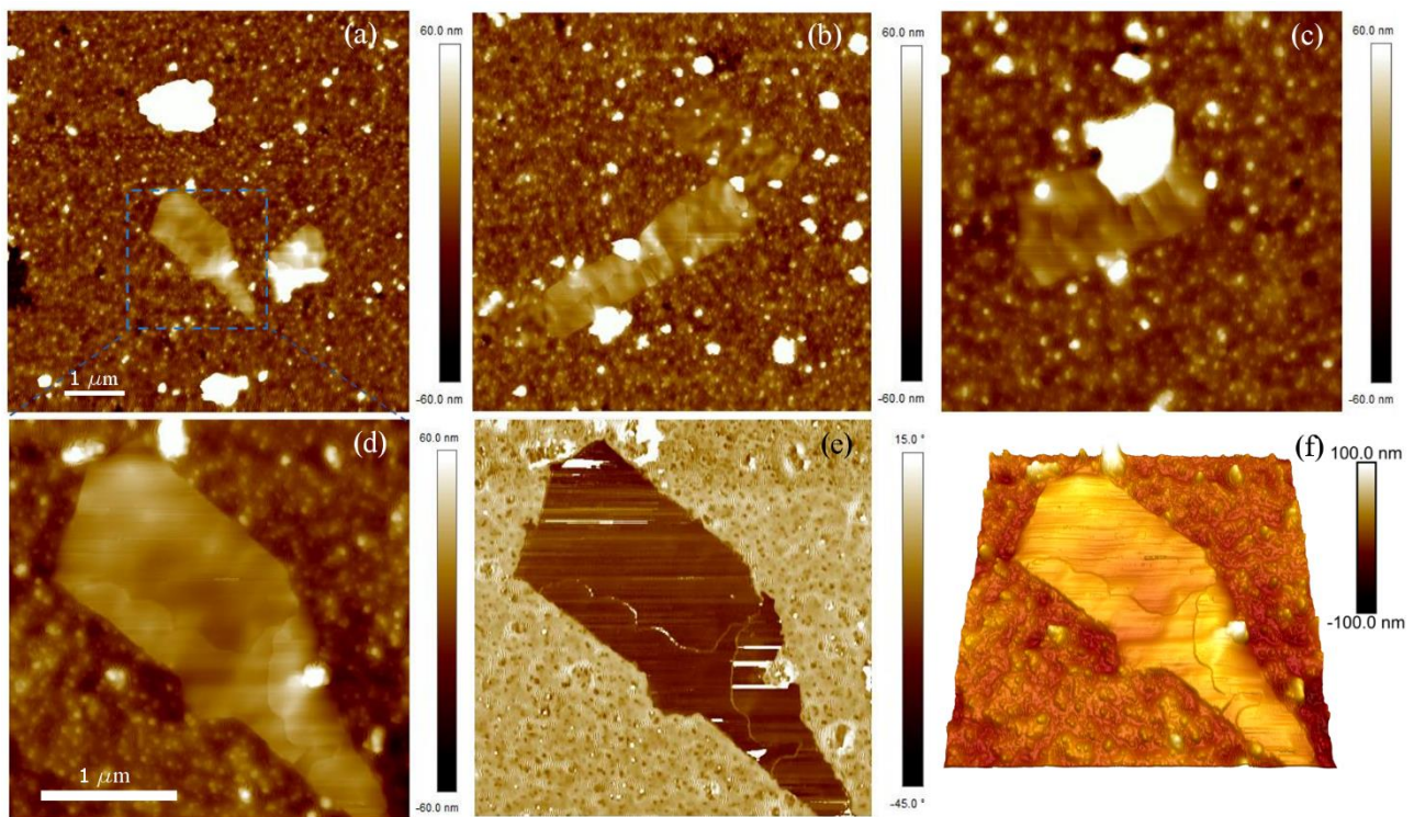
Figure 4. (a-c) AFM morphological maps of a ns-C thin film (SMP1) covered by 10 \mu l of [Bmim][NTf 2 ]/methanol solution; structured [Bmim][NTf 2 ] surrounded in its liquid phase are reported. In d-e-f the AFM top-view, phase map and 3D reconstruction of the structured ionic liquid shown in Figure 4.a are shown.
