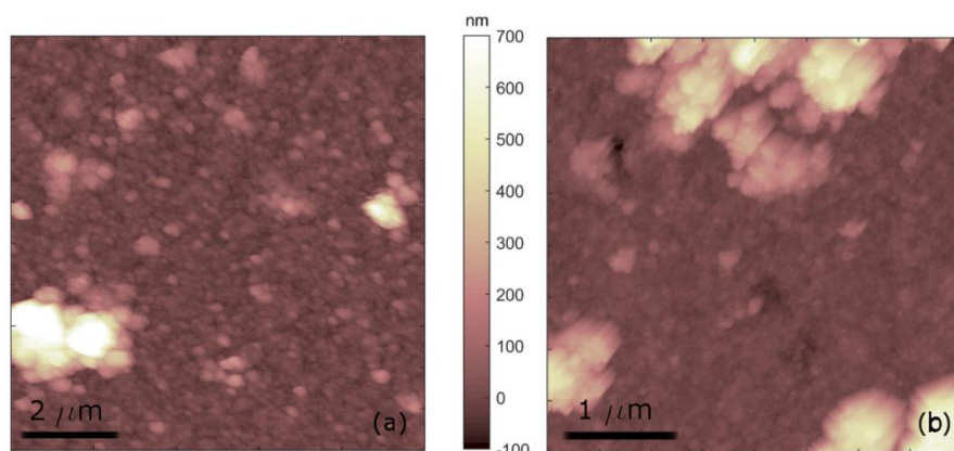
Figure 2. (a) Top-view AFM morphological map of as-deposited ns-C thin films SMP2 and (b) the same sample after the deposition of 300 \mu\text{l} of [Bmim][NTf 2 ]/methanol diluted solution onto it.
